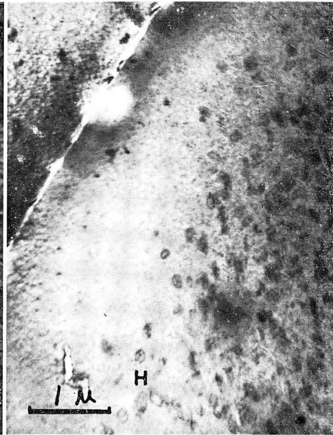
Photo. 48 Al-20% Ag alloy, W.Q., aged for 0.5 hrs at 200°C. ×15000
