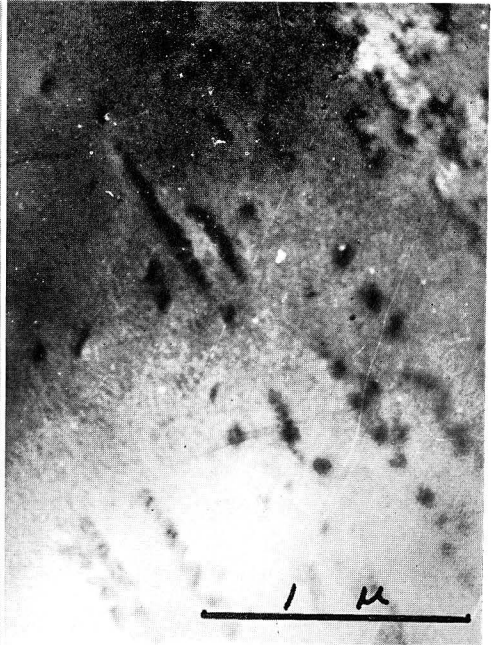
Photo. 20 Al-4% Cu alloy, W.Q., 4.0% elong., aged for 2 days at 70°C. \times 35000
