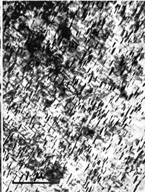
Photo. 50 Al-20% Ag alloy, W.Q., 20% rolled, aged for 4 hrs at 200°C. ×20000
