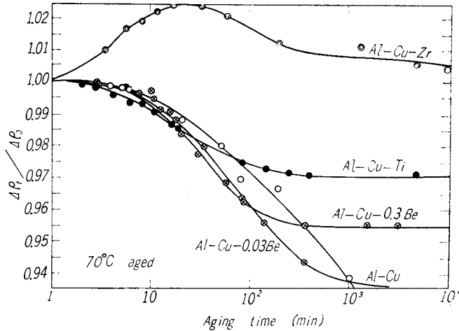
Fig. 7. Isothermal aging curves of resistivity at 70°C in binary and ternary Al-4% Cu alloys.
