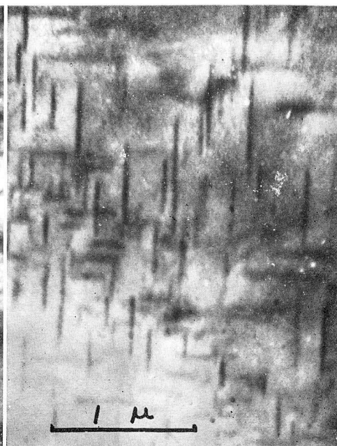
Photo. 26 Al-4% Cu alloy, W.Q., aged for 6 days at 160°C. \times 27000
