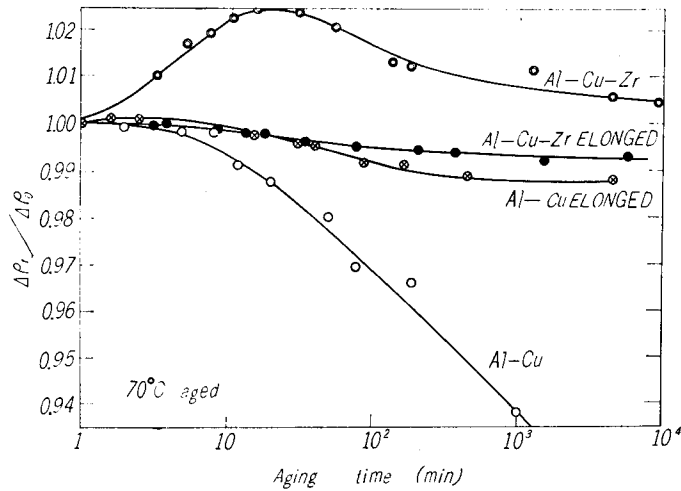
Fig. 9. Effects of cold working on resistivity changes in Al-4% Cu and Al-Cu-Zr alloys during aging at 70°C.
