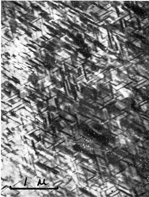
Photo. 47 Al-Ag-Zr alloy, W.Q., 20% rolled, aged for 4 days at 110°C. ×20000
