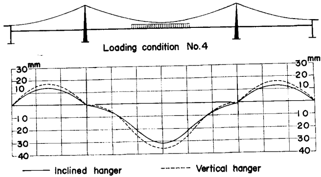
Fig. 4. Static deflectional curves (Loading condition No. 4).
