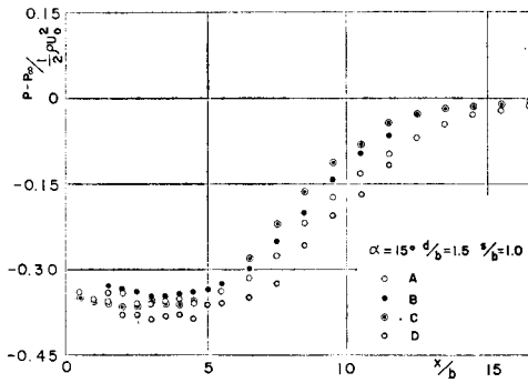
Fig. 7. Static pressure distribution along the walls for a constant step height. ( S/b=1.0 )
