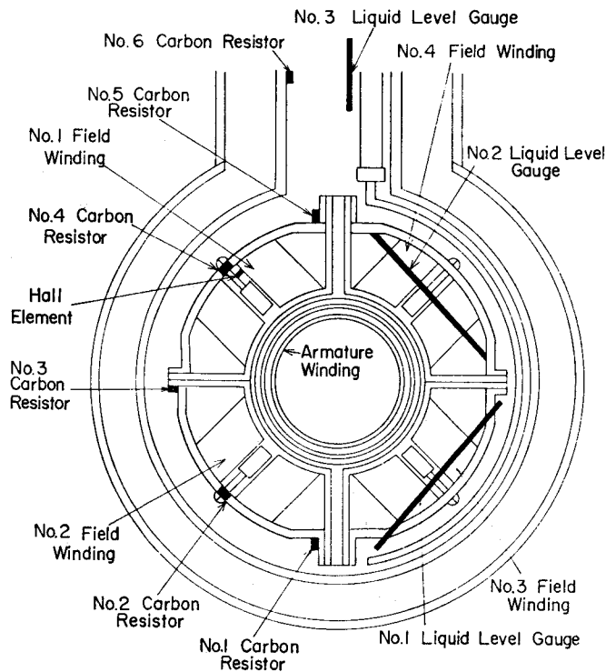
Fig. 2 Detail Cross-Section of the Stator (Cryostat).
