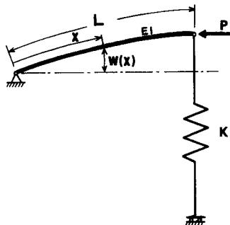
Fig. 3.2. Unstable symmetric buckling model.
