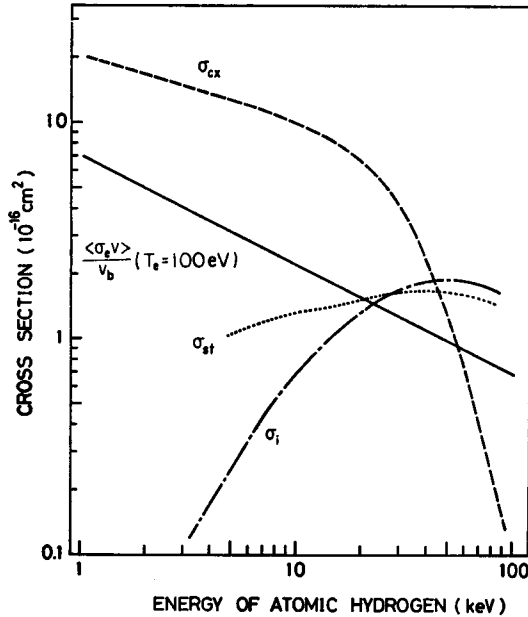
Fig. 2. Cross sections of atomic hydrogen for charge transfer with proton \sigma_{ct} , ionization by proton impact \sigma_i , ionization by electron impact \langle \sigma_e v \rangle / v_b , and charge stripping by molecular hydrogen \sigma_{st} .
