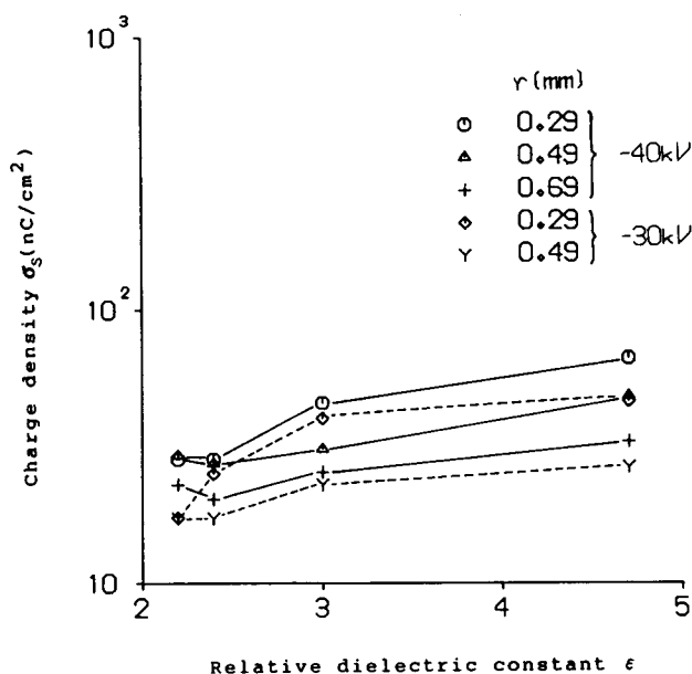
Fig.18 Relation of charge density vs. relative dielectric constant in SF 6 of 1atm.
