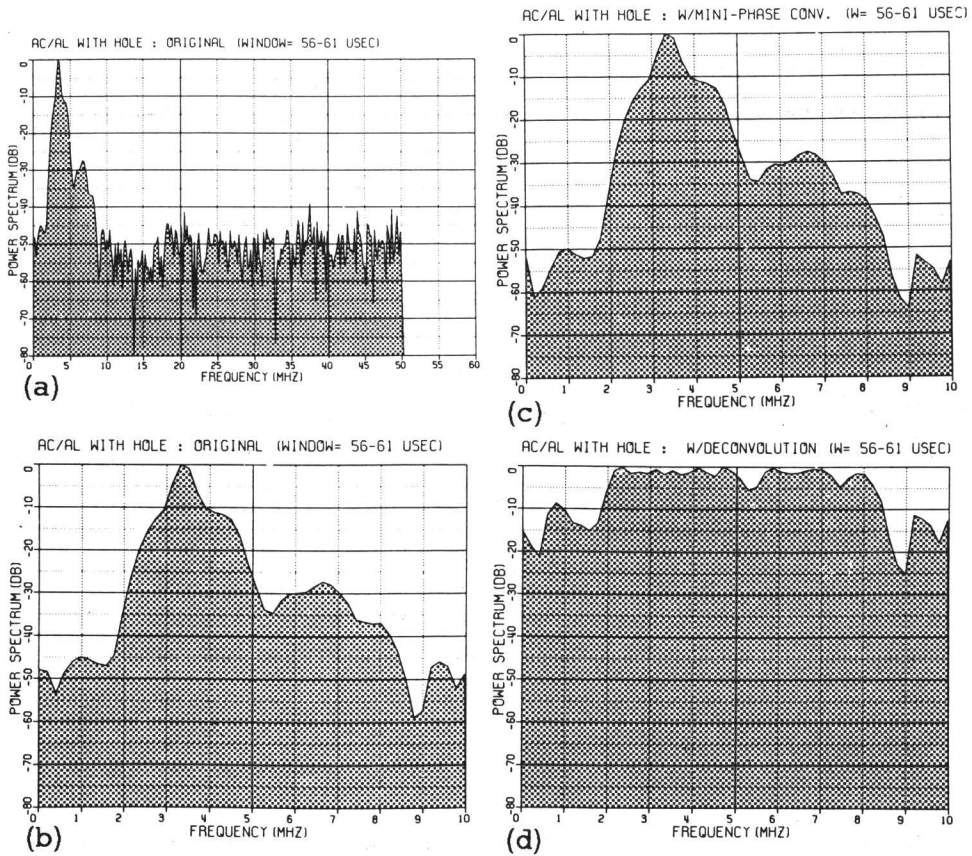
Fig. 4 Power Spectra
