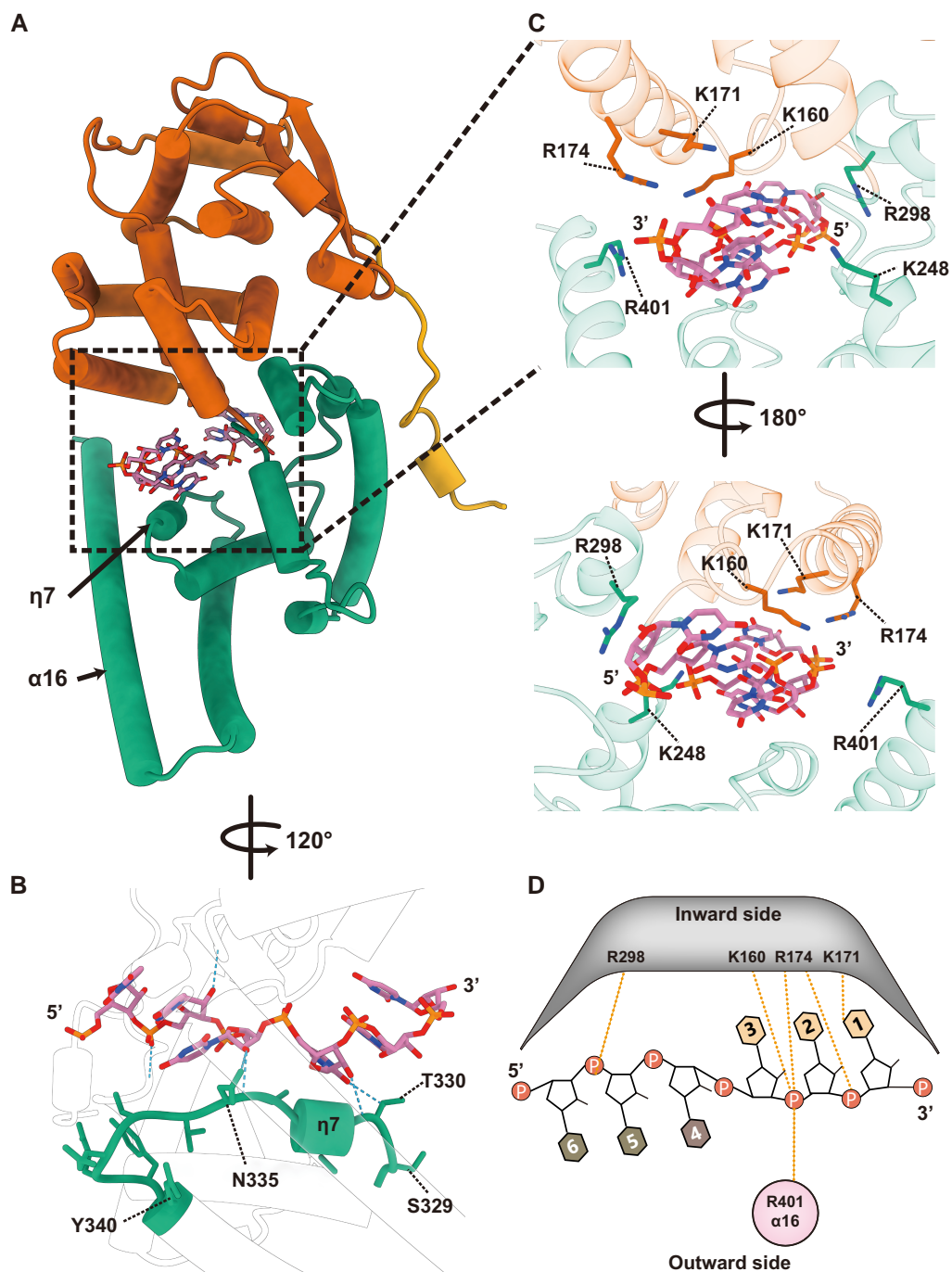
Fig. 2. NP-RNA interactions in the helical NP(full)-RNA complex. (a) The overall structure of the protomeric NP(full)-RNA complex in cylindrical presentation (colored the same as Fig. 1a). (b) Close-up view of the RNA binding site. Hydrogen bonds (distance < 4 \text{ \AA} ) were detected by ChimeraX (35) and shown as blue dotted lines. (c) Close-up view of the RNA binding site. Positively charged amino acids are marked. (d) Schematic diagram of the NP-RNA interactions. The RNA bases are numbered in the 3' to 5' direction. The RNA bases on the helix, facing inward (light-orange) and outward (light-brown). Secondary structure labels are based on our atomic model. Orange dotted lines represent the potential interactions between the NP residues and RNA backbone.
