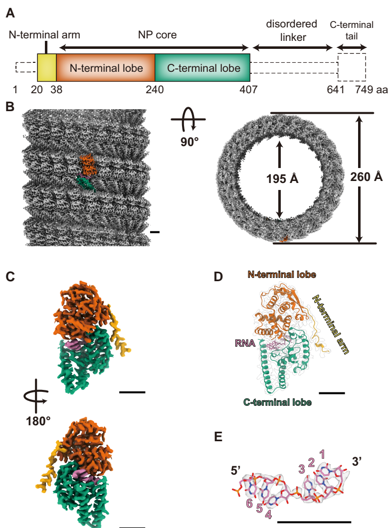
Fig. 1. Overall cryo-EM structure of the LLOV NP(full)-RNA helix and its atomic model. (a) Schematic diagram of the domain architecture of the LLOV NP. Each domain is represented by a unique color, and the unsolved region is represented by a dotted outline. (b) The cryo-EM map of the NP(full)-RNA complex. A single NP-RNA protomer is highlighted with colors: RNA strand in purple and NP in red, green, and yellow, according to the color code shown in (a). (c) The isolated cryo-EM map of the NP-RNA protomer. (d) The atomic model of the NP-RNA complex in ribbon presentation superimposed on the electron microscopy map. (e) The isolated cryo-EM map and atomic model of RNA. RNA bases are modeled as uracil. Scale bar, 20 Å.
