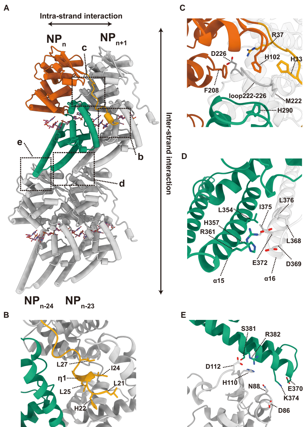
Fig. 3. NP-NP interactions in the helical NP(full)-RNA complex. (a) Four adjacent NP-RNA complexes in a helix. The NP n is colored according to the colors in Fig. 1a. The larger and smaller rectangles with dotted lines highlight (b, c, and d) the close-ups of intrastrand NP-NP interactions between NP n and NP n+1 and (e) interstrand NP-NP interactions between NP n and NP n-24 . (b) NP-NP interactions between the N-terminal arm (yellow) of the NP n and the hydrophobic pocket of NP n+1 (gray). (c) NP-NP interactions between the nut structure formed by the N-terminal arm (yellow), N-terminal lobe (red), and C-terminal lobe (green) of the NP n , and the M222 screw structure of the NP n+1 (gray). (d) NP-NP interactions between α15 of NP n (green) and α16 of NP n+1 (gray). (e) Intrastrand NP-NP interactions between the NP n (green) and NP n-24 (gray).
