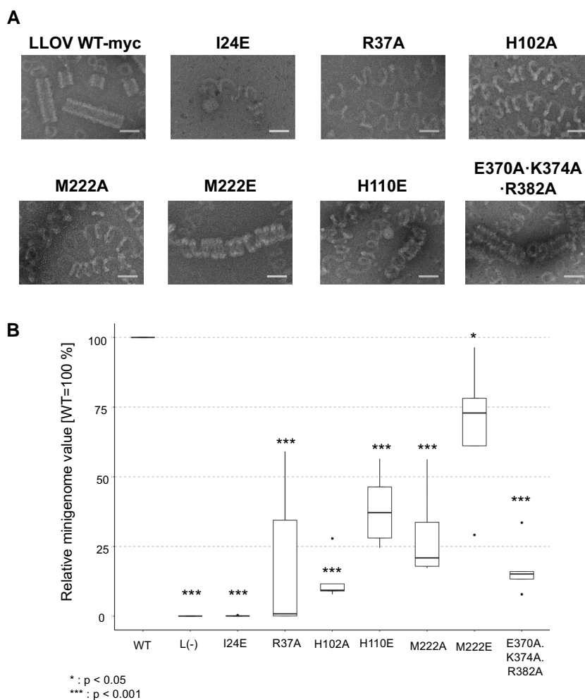
Fig. 4. Structure-based mutational analysis of the LLOV NP. (a) Transmission electron microscopy images of the negatively stained purified helical structure of the LLOV NP(full) mutant–RNA complex. A myc tag was fused to the C-terminus of the native and mutant LLOV NPs. Scale bar, 50 nm. (b) The assessment of the function of the LLOV NP-myc mutants on genome transcription and replication, evaluated via minigenome assays. The experiments were performed in pentaplicates ( n = 5 ). Significance was set at P < 0.05 (*) and P < 0.001 (**).
