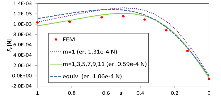
Fig. 5. Speed dependence of thrust force given by conventional approximate equivalent circuit of L-type (“equiv” in the figure); “er.” indicates mean square error compared with FEM.
