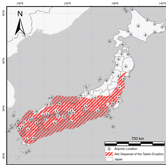
Figure 8. Transformed ash dispersal map using ArcGIS software with airport icons for impacts reference. Human geography base (ESRI, 2022) provided the basemap for this figure.
