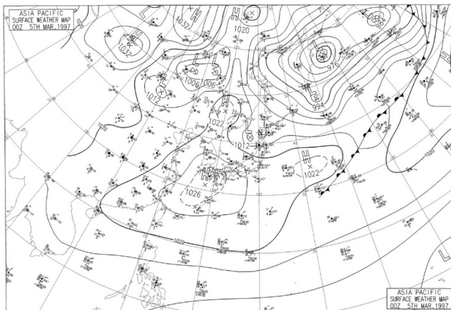
Figure B6. Surface weather chart for Asia Pacific region at 00:00 UTC 5 March 1997. Weather chart image was obtained from the Japan Meteorological Agency (Database of Weather Charts for Hundred Years, 2022; Japan Meteorological Agency, 2022).
