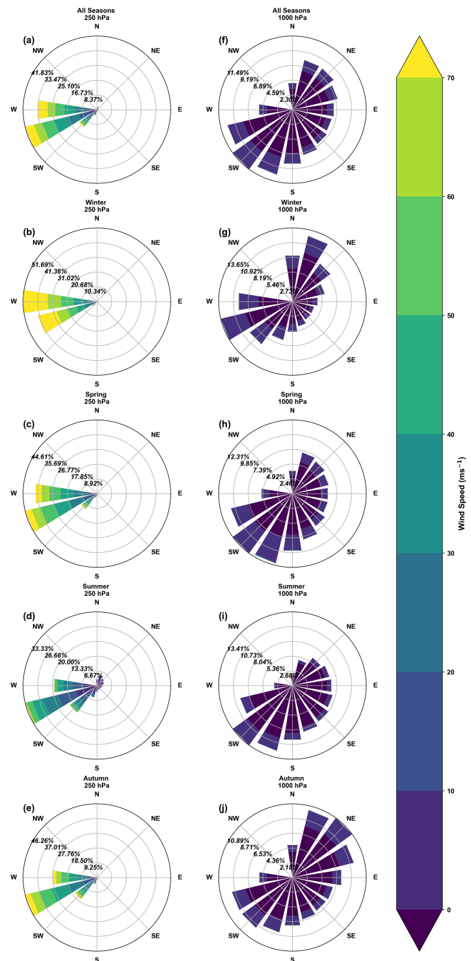
Figure 3. Ten wind roses illustrating wind conditions inferred from the JRA-55 Reanalysis dataset (Kobayashi et al., 2015) for upper altitude winds (first column) and surface winds (second column). (a, f) 1958–2021; (b, g) winter, (c, h) spring, (d, i) summer, and (e, j) autumn. Roses indicate the probability of the provenance and sequential colours indicate the speed gradients.
