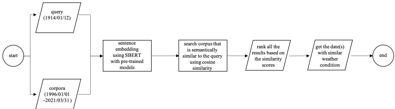
Figure B5. Flowchart for finding dates with weather report commentaries similar to the day of eruption, using a semantic search, based on semantic textual similarity between the old and the modern commentaries, by SentenceBERT (SBERT).
