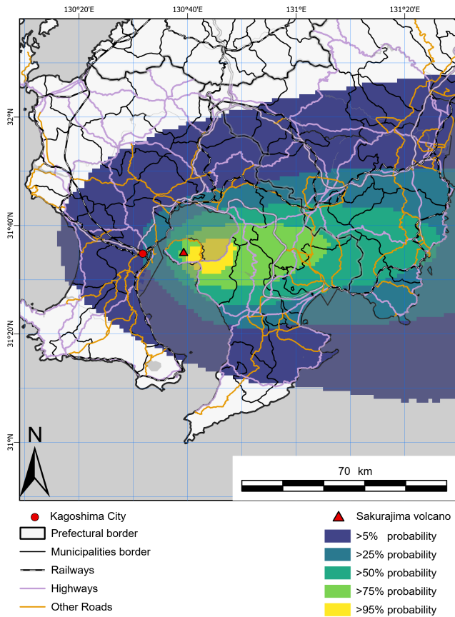
Figure 6. Probability distribution of ash dispersal with the threshold for road closure risk ( \geq 3 cm). Black and white stripes mark railways, and highways and other roads are coloured lines. The colour gradient shows the probability of ash deposits exceeding the threshold. Human geography base (ESRI, 2022) provided the basemap for this figure.
