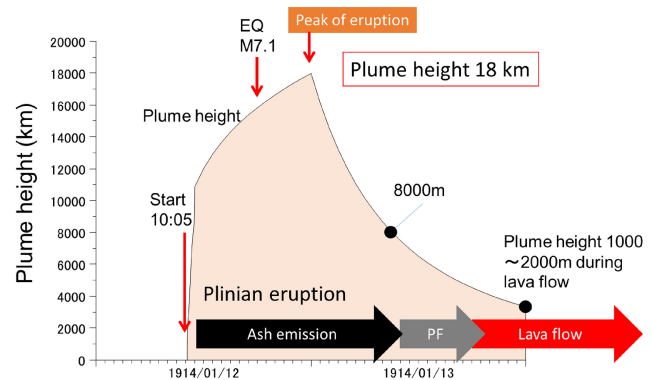
Figure 2. Plume height progression during the Taisho eruption on 12–13 January 1914 with information on both subsequent events and materials ejected. PF means pyroclastic flows that occurred from 13 January 1914 (Takebayashi et al., 2021).
