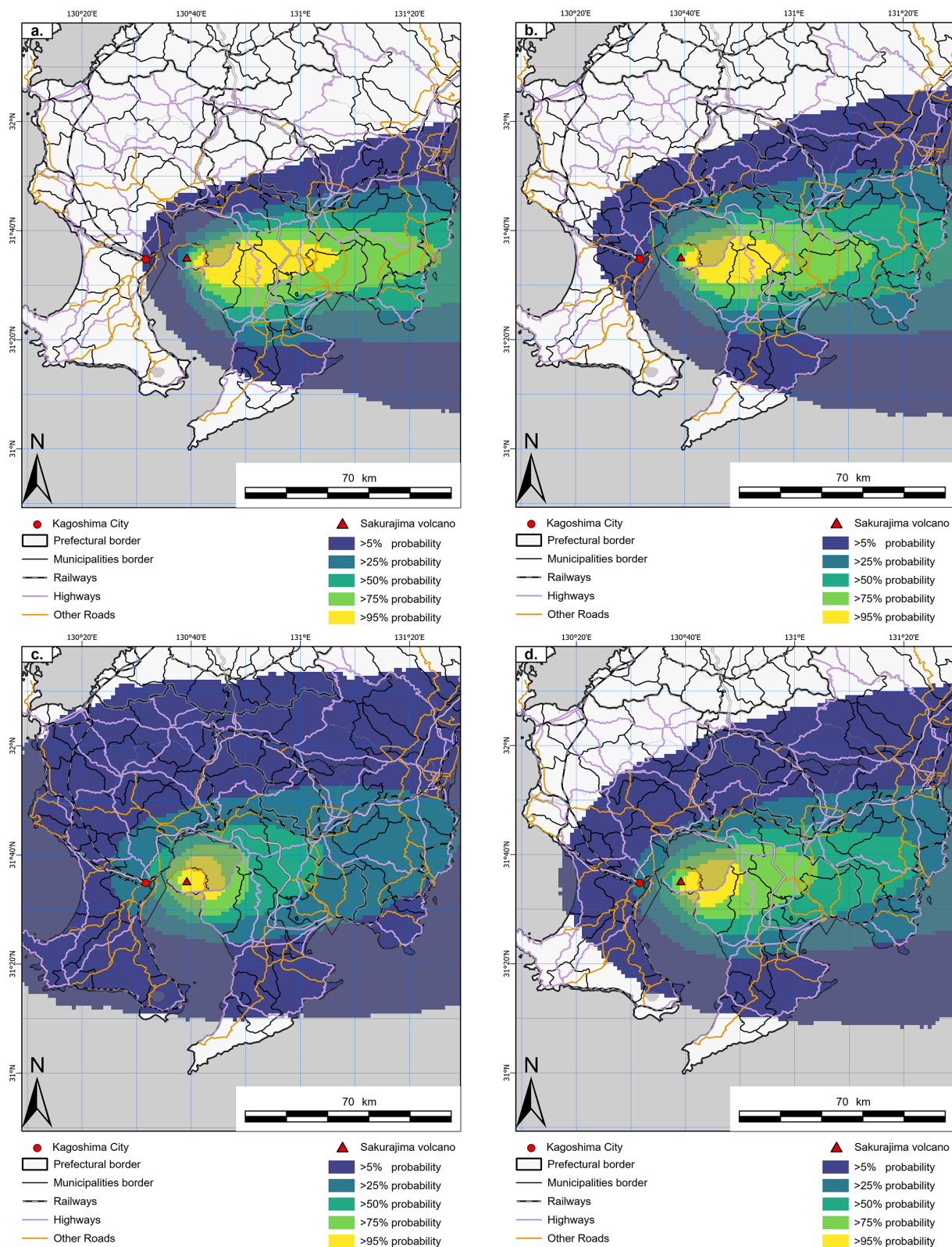
Figure 7. Seasonal probability distribution of ash dispersal with the threshold for road closure risk ( \geq 3 cm). The panels show the probability distribution of ash dispersal during (a) winter, (b) summer, (c) spring, and (d) autumn. Black and white stripes mark railways on the map, and highways and other roads are coloured lines. The colour gradient shows the probability of ash deposits exceeding the threshold. Human geography base (ESRI, 2022) provided the basemap for this figure.
