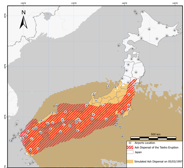
Figure 9. Comparison of ash distribution on the selected date (5 March 1997) according to the original ash dispersal map and simulation results. Human geography base (ESRI, 2022) provided the basemap for this figure.
