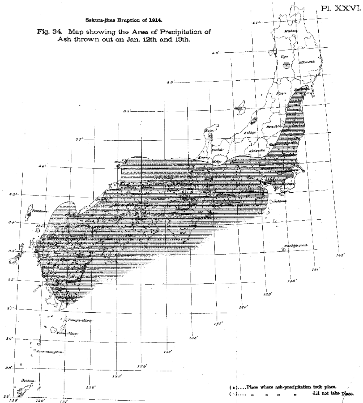
Figure 1. Map of ash dispersal over all of Japan following the Taisho eruption (Omori, 1914).
