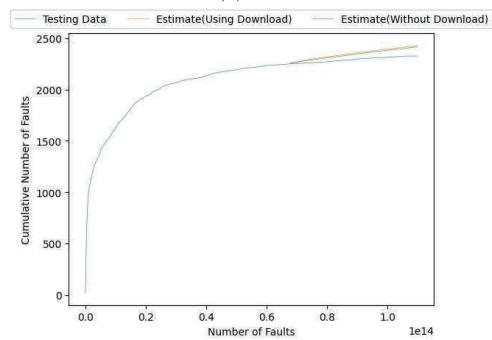
(c) webpack.
