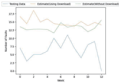
(c) webpack.
