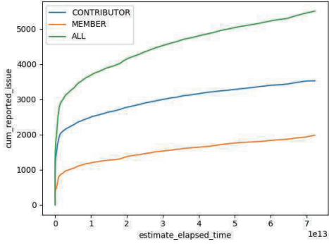
(a) Nx.
