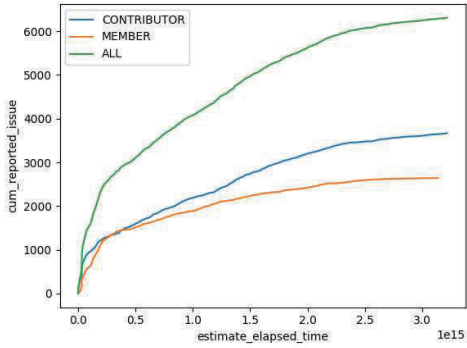
(c) webpack.
