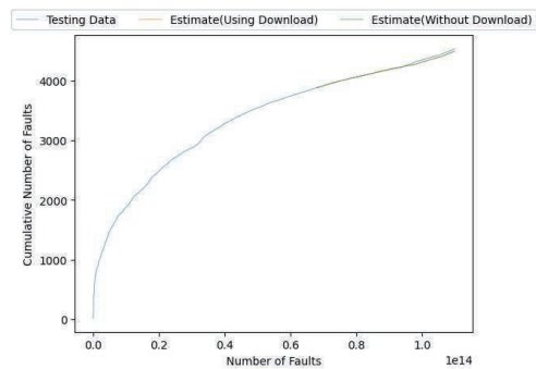
(a) Nx.
