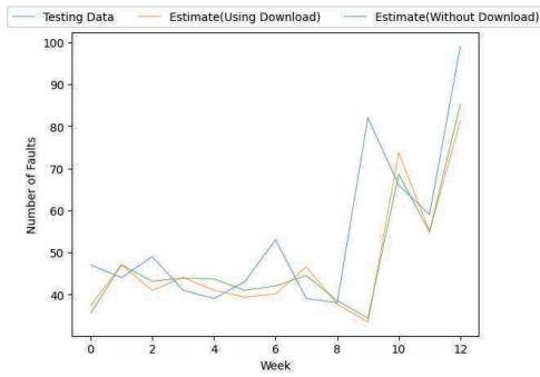
(a) Nx.
