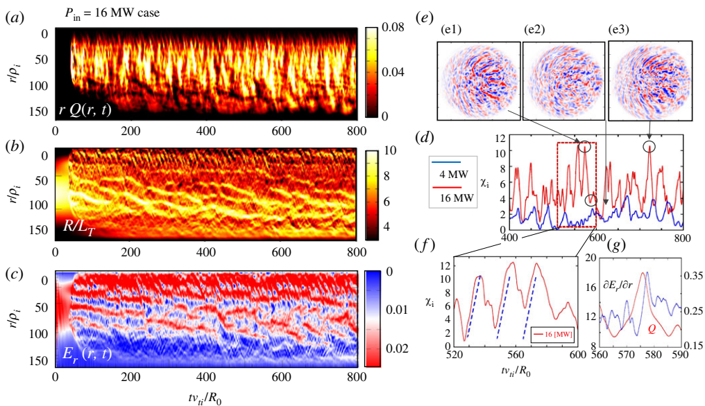
Figure 4. Evolution of distribution in (r, t) plane for (a) heat flux rQ_{\text{tur},b} , (b) temperature scale length R_0/L_T and (c) radial electric field shear E_r for P_{\text{in}} = 16 MW in the case with form factor shown in figure 2b, i.e. \nu_* = 0.42 in the core region. (d) Corresponding radially averaged heat diffusivity \chi_i , (f) Heat diffusivity \chi_i averaged in 520 \leq t \leq 600 and (g) heat flux Q as well as radial electric field shear \partial E_r / \partial r . (e) Represents potential contour plots on poloidal cross-section at times that the heat diffusivity \chi_i becomes peak values for (e1) and (e3) while a bottom value for (e2). (Online version in colour.)
