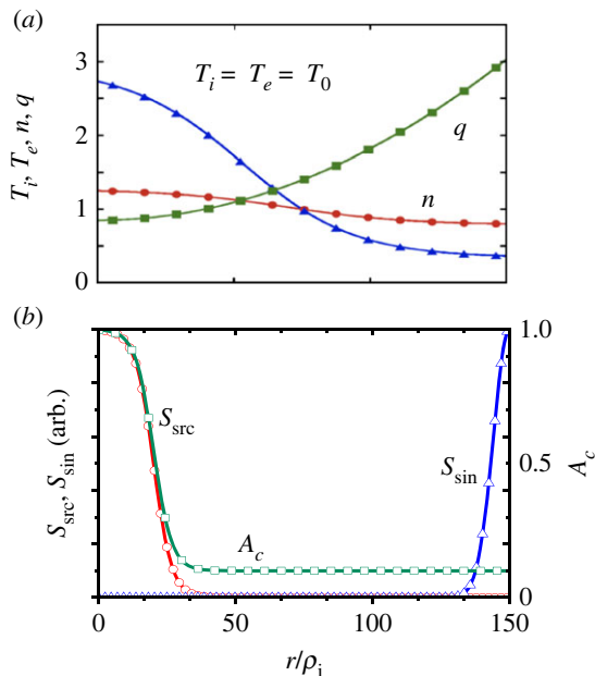
Figure 2. (a) Initial temperature and density profiles, T_i(r) and n_i(r) , and safety factor profile q(r) . (b) Profile of heating source and sink, i.e. S_{src} and sink S_{sik} , and that of the form factor of the collisionality, \nu_{col}(r) . (Online version in colour.)
