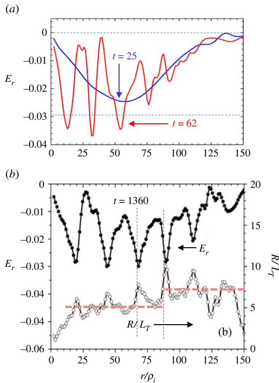
Figure 7. (a) Distribution of radial electric field E_r before linear ITG mode grows at t = 25 and after the mode saturates at t = 62 , (b) distribution of E_r ( < 0 ) and R/L_T in the quasi-steady state at t = 1360 (data from [33]). (Online version in colour.)
