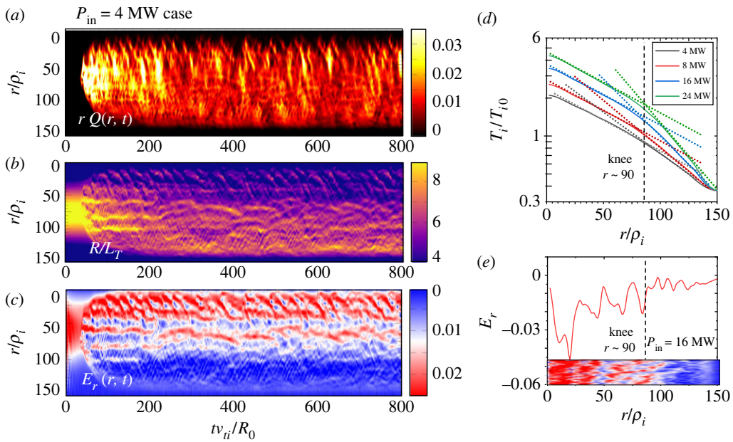
Figure 3. Evolution of distribution in (r, t) plane for (a) heat flux rQ_{\text{tur},b} , (b) temperature scale length R_0/L_T , (c) radial electric field shear E_r for P_{\text{in}} = 4 MW in the case with the form factor shown in figure 2b, i.e. \nu_* = 0.42 in the core region. (d) Established temperature profiles in the quasi-stationary state for different input power of P_{\text{in}} = 4, 8, 16, 24 MW. Each profile has an exponential function fit, the scale lengths of which are changed at r \sim 90 defined by 'knee'. (e) Distribution of E_r for P_{\text{in}} = 16 MW, which corresponds to that in (d) and also figure 4, in which collisionality is also \nu_* = 0.42 in the core region. In (e), the dynamics of E_r is also inserted in 300 \leq t \leq 600 for reference. (Online version in colour.)
