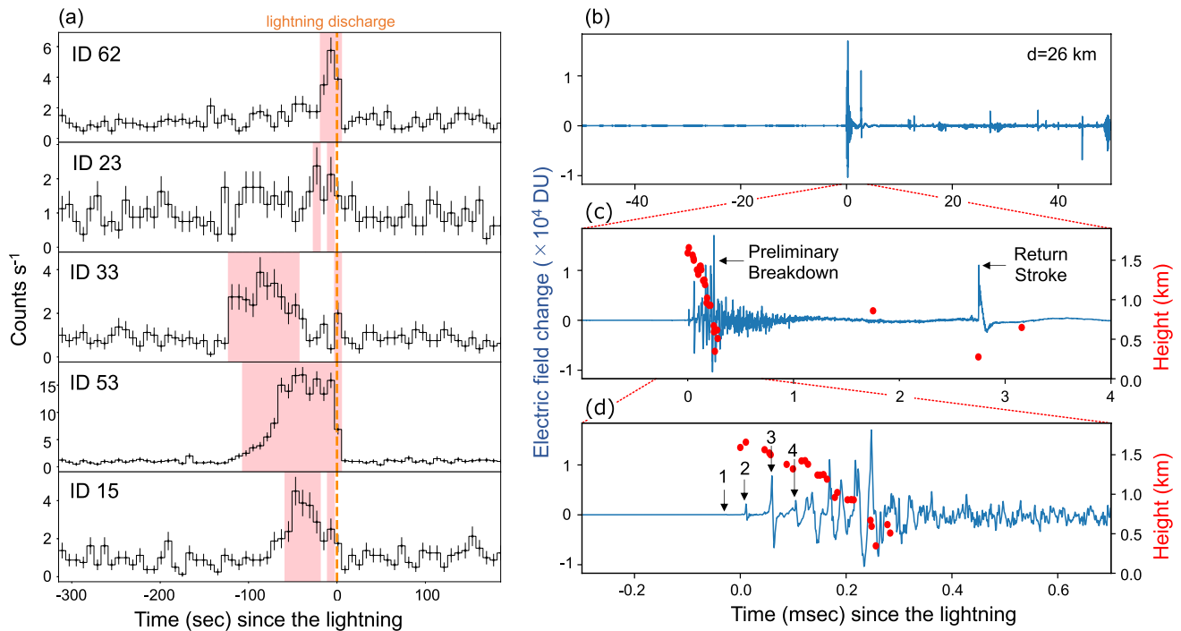
Figure 2. (a) 8-s-binned count rate histories of radiation in the 3–10 MeV band recorded by five Cogamo detectors of, from the top to bottom panels, Cogamo IDs 62 (36.57°N, 136.65°E), 23 (36.57°N, 136.65°E), 33 (36.56°N, 136.65°E), 53 (36.56°N, 136.65°E), and 15 (36.55°N, 136.65°E), in the order of the north to south. Error bars are statistical 1\sigma . The time origin is 04:08:34.8565 JST on 30 December 2021, which corresponds to the first signal of the lightning discharge recorded by FALMA and DALMA. Data bins with detection significance exceeding 3.5\sigma are marked in red. (b–d) Preliminary breakdown pulses recorded by FALMA (blue lines, the left vertical axis) and their heights mapped by DALMA (red markers, the right axis). The time origin is the same as panel (a). The four pulses with numbers indicated are used for the location analysis.
