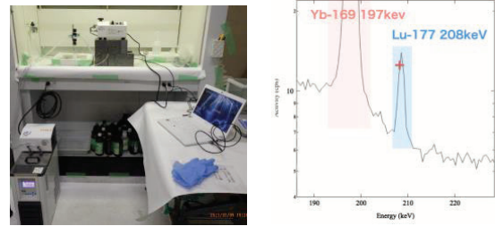
Fig. 2. Experimental set-up for separation of Lu-177 from Yb-176.
