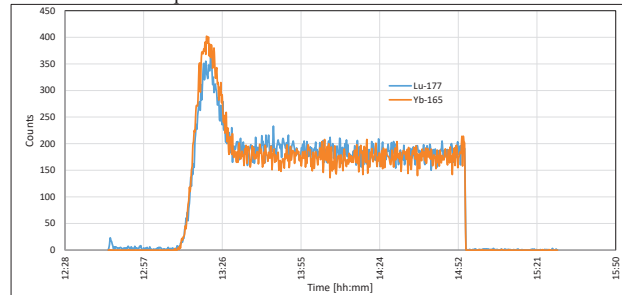
Fig. 3. Elution profile of extraction chromatography with an 11 mm \phi × 240 mL column packed with LN2 resin measured with a CZT detector.
