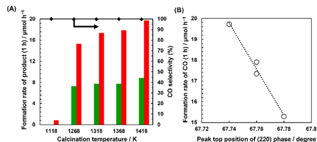
Fig. 5 (A) Formation rates of CO (red), \text{H}_2 (blue), and \text{O}_2 (green) and the selectivity toward CO evolution (black diamond) in the photocatalytic conversion of \text{CO}_2 in \text{H}_2\text{O} over Ag-Co/ \text{Mg-SrTiO}_3 _x K photocatalysts ( x = 1118, 1268, 1318, 1368 , and 1418 ). Reaction conditions: amount of photocatalyst: 0.2 g; Ag loading: 1 wt%; Co loading: 0.3 wt%; volume of reaction solution ( \text{H}_2\text{O} ): 0.2 L; additive: 0.1 M \text{NaHCO}_3 ; \text{CO}_2 flow rate: 30 \text{ mL min}^{-1} ; light source: monochromatic LED lamp at 365 nm; photoirradiation time: 1 h. (B) Dependence of peak position on CO formation rate.
