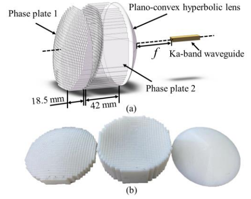
Fig. 5. (a) Schematic of experimental setup for verification of reconfigurable prism concept. (b) The prototype of the proposed decentered phase plate and plano-convex hyperbolic lens with PLA plastic material.
