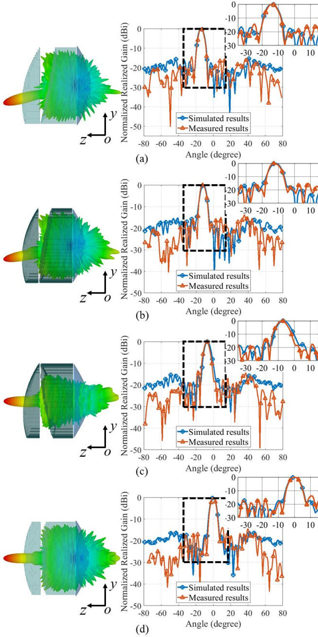
Fig. 6. The radiation performance of reconfigurable prism concept operating at 30GHz with two decentered phase plates at different rotation angle. (a) \theta_{r1} = 0^\circ, \theta_{r2} = 0^\circ . (b) \theta_{r1} = 30^\circ, \theta_{r2} = -30^\circ . (c) \theta_{r1} = 60^\circ, \theta_{r2} = -60^\circ . (d) \theta_{r1} = 90^\circ, \theta_{r2} = -90^\circ .
