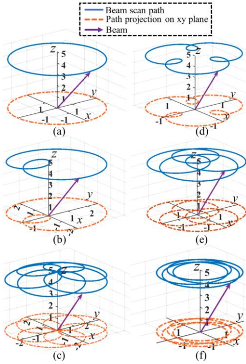
Fig. 2. The set of generated scan patterns by using prisms with different prism angles at different rotational speed. (a) M = 1, N = 1 . (b) M = 1, N = 2 . (c) M = 1, N = 6 . (d) M = 0.5, N = 4 . (e) M = 1.5, N = 4 . (f) M = 5, N = 4 . Noted that the ratio of prism angle for two prisms is M = \delta/\delta' , and the ratio of rotational speed for two prisms is N = \omega/\omega' .
