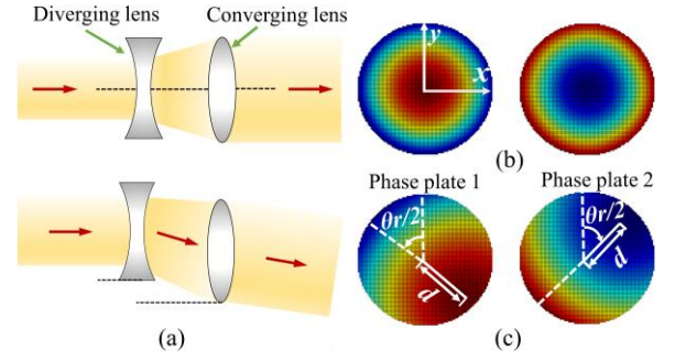
Fig. 3. (a) The beam deflection in a specific direction like a prism using Galilean afocal lens pair system with opposite optical powers. (b) Schematic of phase distribution for the lens pair with opposite optical powers. Left: diverging lens; Right: converging lens. (c) Schematic of the corresponding decentered phase distribution.
