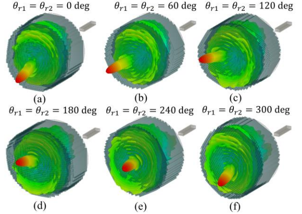
Fig. 7. The simulated 3-D radiation patterns of reconfigurable prism concept operating at 30GHz by rotating two phase plates along the same direction with the same angle (a) \theta_{r1} = \theta_{r2} = 0^\circ . (b) \theta_{r1} = \theta_{r2} = 60^\circ . (c) \theta_{r1} = \theta_{r2} = 120^\circ . (d) \theta_{r1} = \theta_{r2} = 180^\circ . (e) \theta_{r1} = \theta_{r2} = 240^\circ . (f) \theta_{r1} = \theta_{r2} = 300^\circ .
