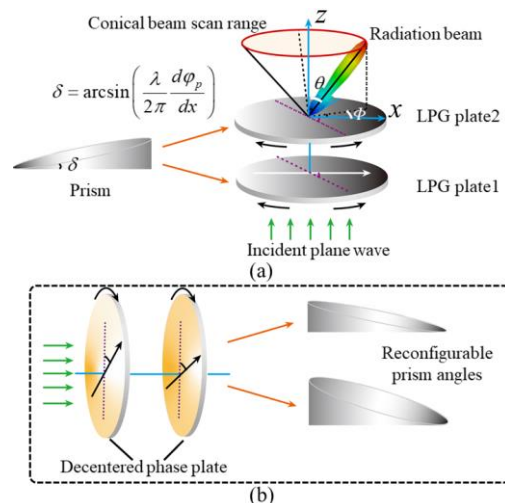
Fig. 1. (a) The typical Risley prism antenna system with a pair of rotating linear phase gradient plate. The white arrow represents the direction of linear phase gradient (b) Schematic diagram of proposed rotationally reconfigurable single-element prism. Different prism angles can be realized by rotating a pair of decentered phase plate.
