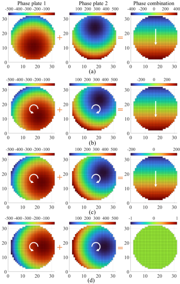
Fig. 4. Different combinations of phase distribution of two decentered phase plates operating at 30GHz with different rotation angle ( \theta_{r1} = \theta_r/2 and \theta_{r2} = -\theta_r/2 ). (a) \theta_{r1} = 0^\circ, \theta_{r2} = 0^\circ . (b) \theta_{r1} = 30^\circ, \theta_{r2} = -30^\circ . (c) \theta_{r1} = 60^\circ, \theta_{r2} = -60^\circ . (d) \theta_{r1} = 90^\circ, \theta_{r2} = -90^\circ .
