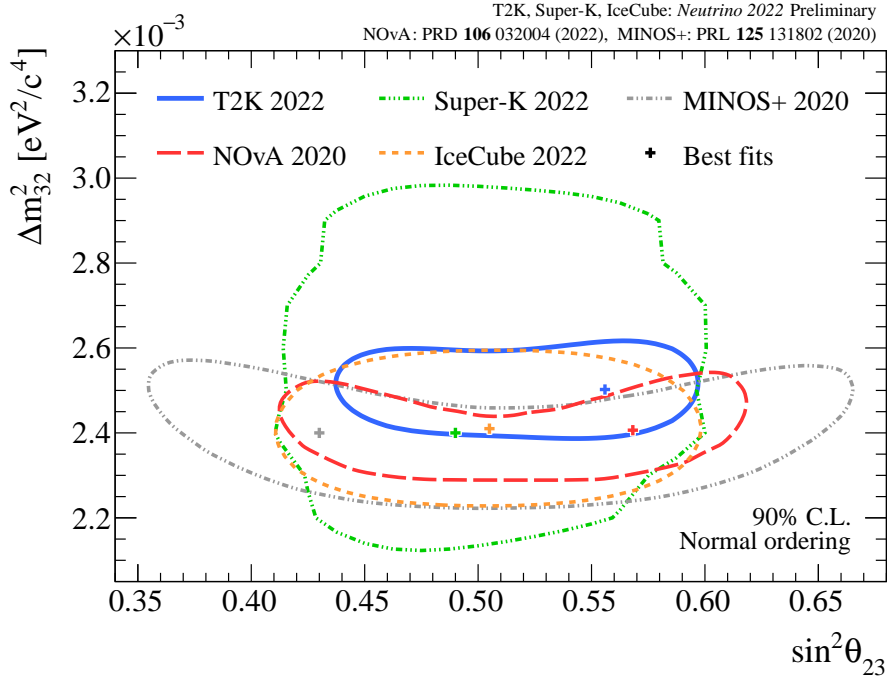
Figure 42: Comparisons of the constraints on the oscillation parameters in the \sin^2 \theta_{23}-\Delta m_{32}^2 plane among the neutrino oscillation experiments. In addition to the updated result from the T2K experiment, Super-Kamiokande experiment [149,150], NO \nu A experiment [152,153], IceCube experiment [154] and MINOS+ experiment [151] are shown. The computing methods are different among experiments. The NO \nu A and IceCube constraints are produced with the Feldman and Cousins (FC) method while the constraints from the other experiments are computed with the fixed \Delta\chi^2 method. The treatments of the mass ordering are also different. The NO \nu A experiment takes the minimum over both mass orderings. On the other hand, the other experiments assume the normal mass ordering in creating these contours.
