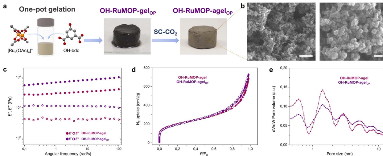
Fig. 5 (a) Schematic representation of the one-pot production of OH-RuMOP-ager OP and its further transformation into OH-RuMOP-ager OP , showing photographs of the resulting materials. (b) FE-SEM images at different magnifications of OH-RuMOP-ager and OH-RuMOP-ager OP . The right part image is the magnification of the corresponding yellow square. The scale bars for the left and right images are 500 and 100 nm, respectively. (c) Storage ( E' ) and loss ( E'' ) Young's modulus for OH-RuMOP-ager OP (purple) compared to OH-RuMOP-ager (magenta). (d) N 2 adsorption (filled circle) and desorption (open circle) at 77 K of OH-RuMOP-ager OP (purple) compared to OH-RuMOP-ager (magenta). (e) Pore size distribution (PSD) of OH-RuMOP-ager OP (purple) compared to OH-RuMOP-ager (magenta) estimated from N 2 isotherms by NLDFT on a slit pore model.
