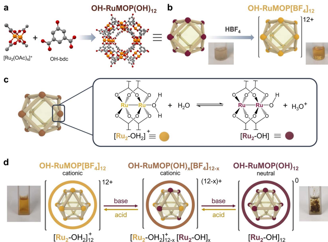
Fig. 1 (a) Schematic representation of the synthesis of OH-RuMOP(OH) 12 from its building blocks. (b) Transformation of non-soluble OH-RuMOP(OH) 12 into soluble OH-RuMOP[BF 4 ] 12 due to the removal of coordinated OH - ligands upon acid treatment with HBF 4 . (c) Acid-base equilibrium between water-coordinated and hydroxo-coordinated Ru 2 (CO 2 ) 4 paddlewheel units in water solutions. (d) Schematic representation of the gradual interconversion between cationic OH-RuMOP[BF 4 ] 12 and neutral OH-RuMOP(OH) 12 upon acid/base treatment.
