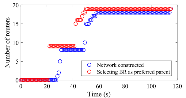
FIGURE 15. Transition of the number of Router connected to BR (star topology, experiment).
