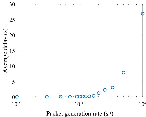
FIGURE 21. Average delay time to successfully transmit packet (fixed large-scale tree topology, 100 router nodes).
