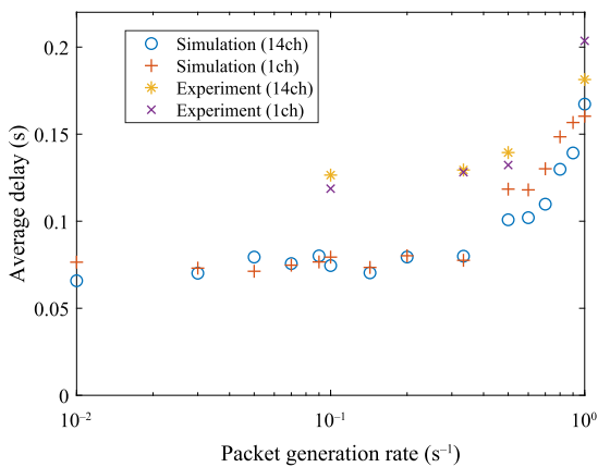
FIGURE 9. Average delay time to successfully transmit packet (star topology).
