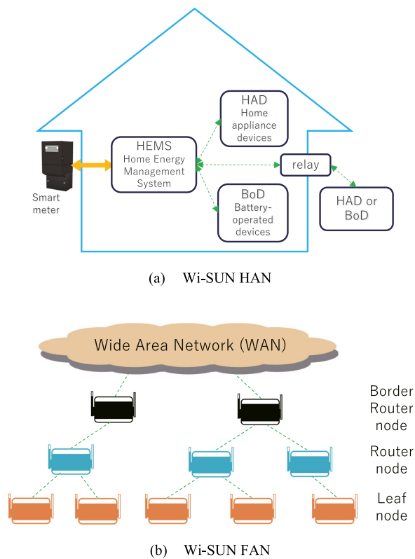
FIGURE 1. Wi-SUN application.
