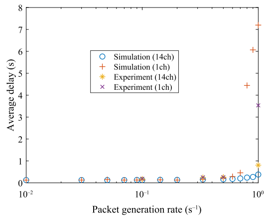
FIGURE 12. Average delay time to successfully transmit packet (tree topology).
