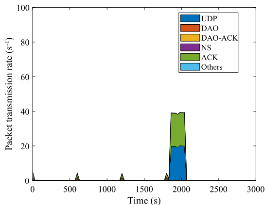
FIGURE 10. Breakdown of the number of packets transmitted per unit time when the packet generation rate is 1.00\text{ s}^{-1} and the number of channels used is one (Star topology, simulation).
