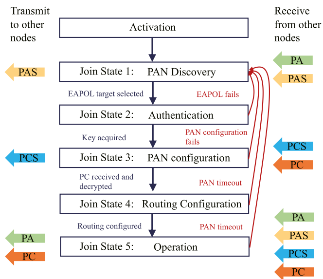
FIGURE 4. Operation of a node in Wi-SUN FAN.
