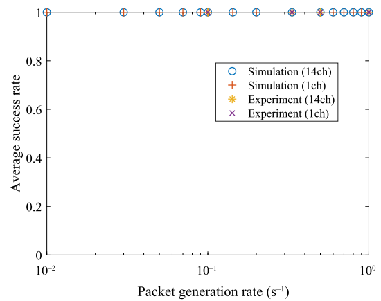
FIGURE 8. Average transmission success rate (star topology).
