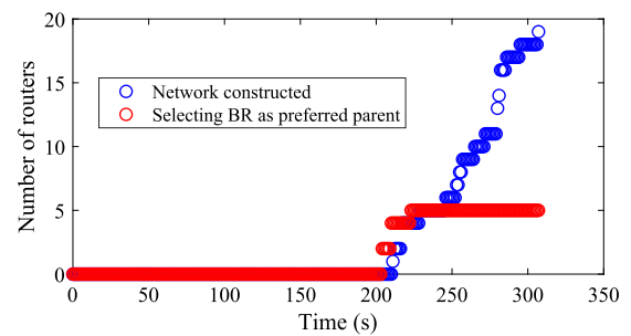
FIGURE 17. Transition of the number of Router connected to BR (tree topology, experiment).
