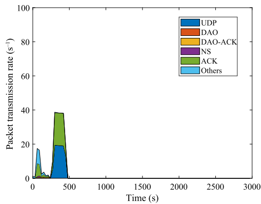
FIGURE 16. Breakdown of the number of packets transmitted per unit time when packet generation rate is 1.00 \text{ s}^{-1} and the number of channels used is one (star topology, experiment).
