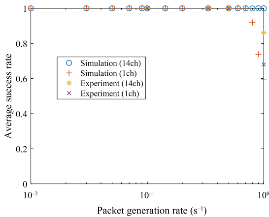
FIGURE 11. Average transmission success rate (tree topology).
