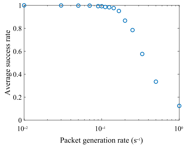
FIGURE 23. Average transmission success rate (a large-scale tree topology assuming for outdoor installation, 100 router nodes).
