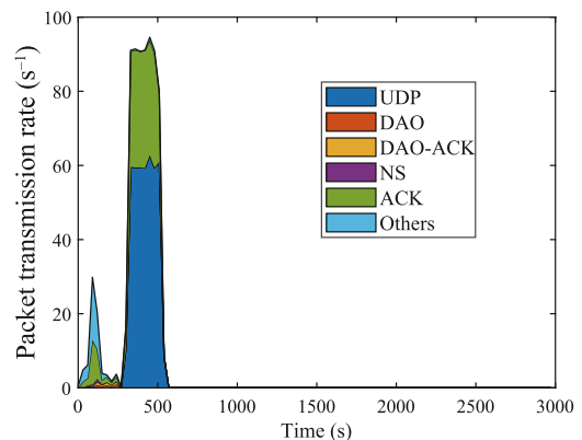
FIGURE 18. Breakdown of the number of packets transmitted per unit time when packet generation rate is 1.00 \text{ s}^{-1} (tree topology, experiment, 14 channels).
