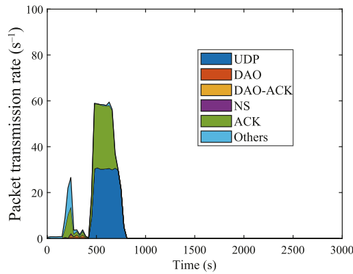
FIGURE 19. Breakdown of the number of packets transmitted per unit time when packet generation rate is 1.00 \text{ s}^{-1} (tree topology, experiment, 1 channel).
