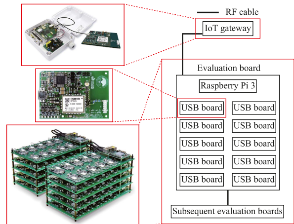
FIGURE 14. Configuration of the Wi-SUN FAN used in the experimental environment.
