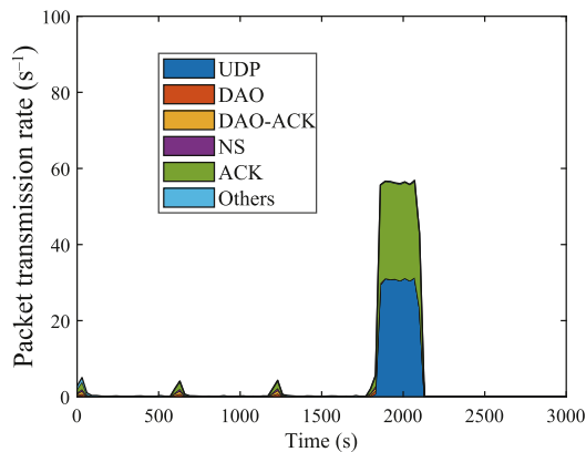
(b) Number of packets sent per unit time (1 channel)
