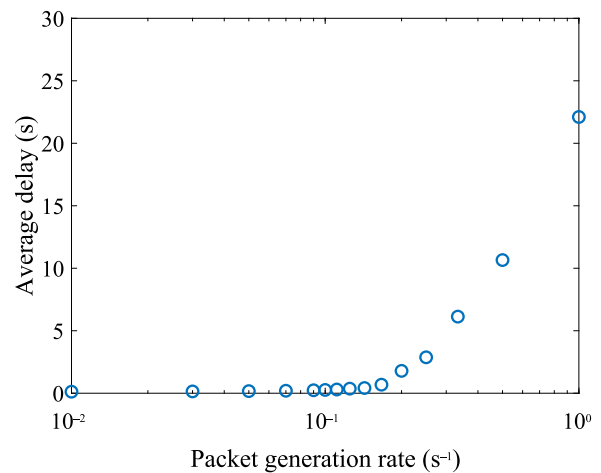
FIGURE 24. Average delay time to successfully transmit packet (a large-scale tree topology assuming for outdoor installation, 100 router nodes).
