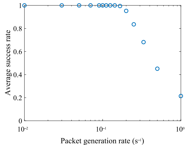
FIGURE 20. Average transmission success rate (fixed large-scale tree topology, 100 router nodes).
