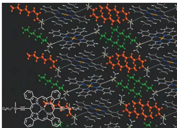
Figure 1. Packing structure of 5,15-bis( n -octyldimethylsilyl)ethynyl tetrabenzoporphyrin in the solution processed thin film.
