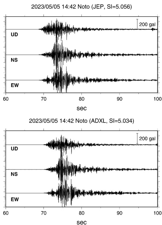
Fig.5 : Waveform of the M6.5 earthquake at 14:42 on 2023/05/05 observed at DP.HRJ. The upper waveform is observed by JEP-8E3 and the lower one by ADXL355.
