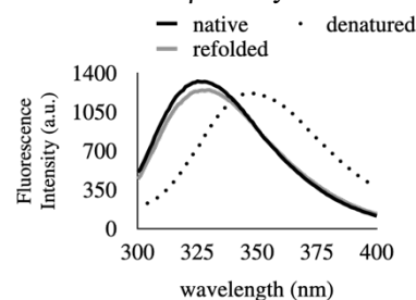
Fig.2. Monitoring of refolding process of low dose ( \sim 5 Gy) irradiated \beta B2-crystallin.
