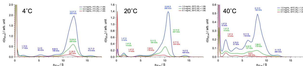
Fig. 1. AUC results of MbHsp17.3 at 4 °C, 25 °C, and 40 °C
