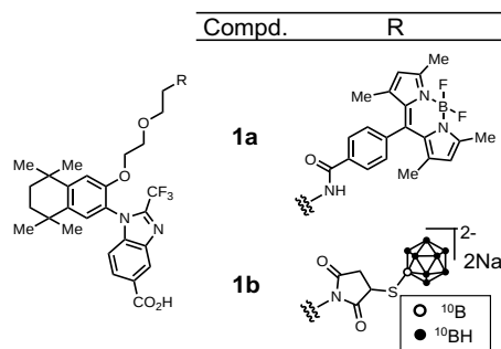
Figure 1. Chemical structures of 1a and 1b .
