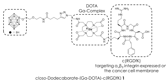
Fig 1. Chemical structure of closo -dodecaborate- 67 Ga[(Ga-DOTA)-c(RGDfK)] ( 67 Ga) 1 .
