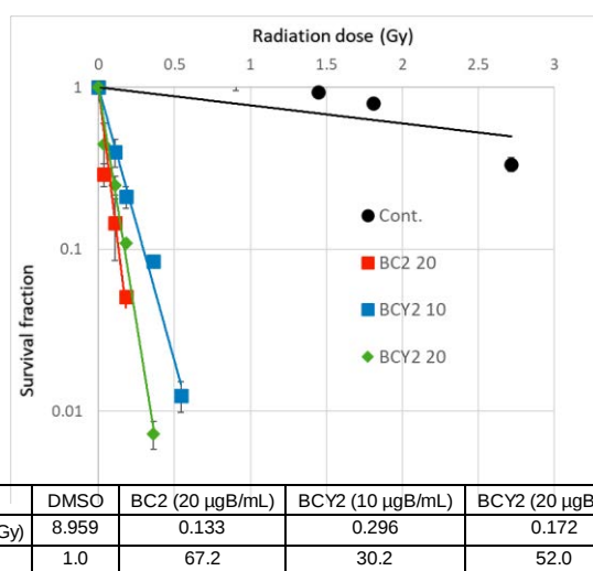
Fig. 2. Survival fraction of T98G cells treated with BC2 and BCY2 with mixed-neutron irradiation.
