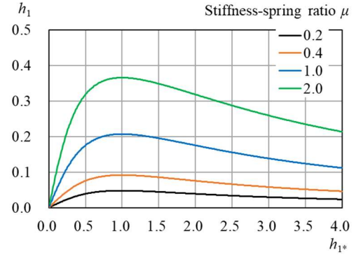
Fig.2 Damping ratio h_1 as a function of the damping ratio h_{1*}
