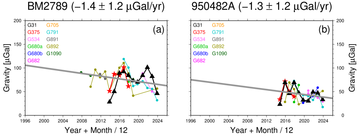
Fig. 3 Relative gravity variations observed at the gravity points far from Sakurajima Volcano. Colored symbols indicate the measured gravity values relative to the SVOG's reference gravity point, and thick gray lines indicate the regression lines to the measured gravity values. The panels of (a) and (b) show the gravity variations at the BM2789 and 950482A gravity points, respectively.
