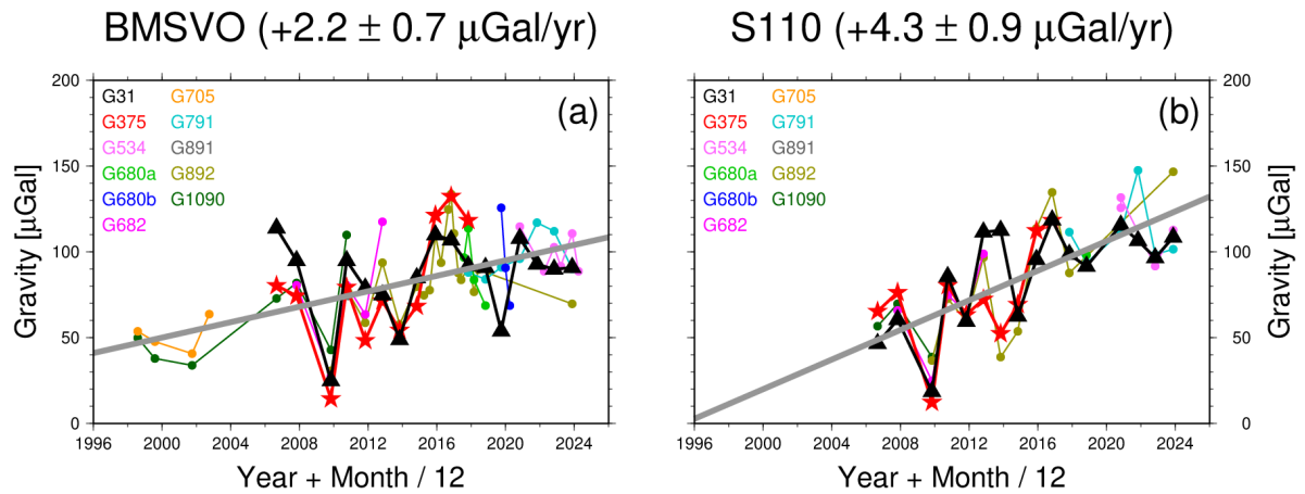
Fig. 2 Relative gravity variations observed at the central part of Sakurajima Volcano. Colored symbols indicate the measured gravity values relative to the SVOG's reference gravity point, and thick gray lines indicate the regression lines to the measured gravity values. The panels of (a) and (b) show the gravity variations at the BMSVO and S110 gravity points, respectively.
