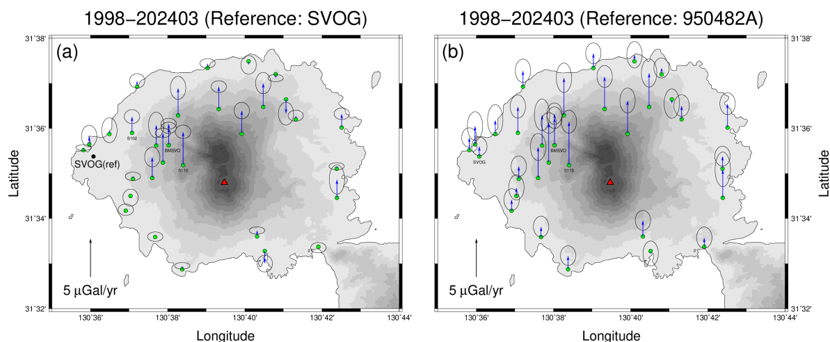
Fig. 4 Spatial distributions of gravity variation rate determined using the relative gravity change observed from 1998 to 2024. Blue arrows and black ellipses indicate the observed gravity variation rate and its standard deviation, respectively. (a) The gravity variation rate relative to the SVOG gravity point located at the western foot of Sakurajima Volcano. (b) The gravity variation rate relative to the 950482A gravity point, which is the farthest gravity point from Sakurajima Volcano.
