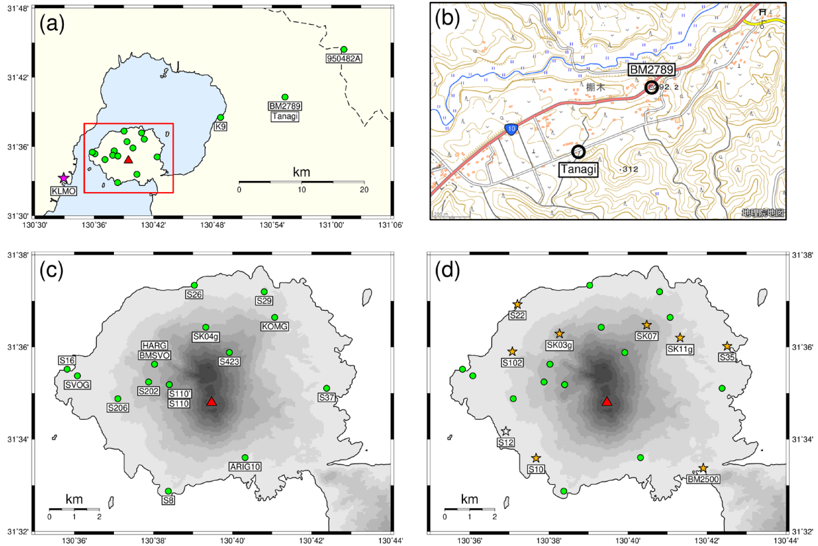
Fig. 1 Gravity points around Sakurajima Volcano. (a) The wide-area map around Sakurajima Volcano. Green circles and red triangles indicate the regular gravity points and Minami-dake Crater, respectively. A pink star, a red rectangle, and a dashed line indicate the location of the weather station at Kagoshima Local Meteorological Observatory (KLMO), the area of the panels (c)–(d), and the boundary between Kagoshima and Miyazaki Prefectures, respectively. (b) The topographic map of the Tanagi region, Soo City, provided by Geospatial Information Authority of Japan. Circles indicate the gravity points in the Tanagi region. (c)(d) Topographic maps of Sakurajima Volcano, contoured every 100 m altitude using the topographic data provided by Geospatial Information Authority of Japan. Green circles indicate the regular gravity points where we measured gravity values in FY2022 and FY2023. Orange stars indicate the additional gravity points where we measured gravity values in FY2023, for the first time in the last 10 years. A white star is the S12 gravity point, where we gave up measuring gravity in FY2023.
