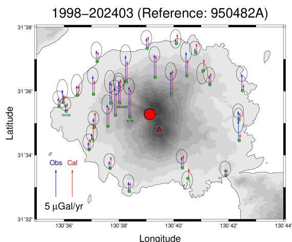
Fig. 5 Gravity variations due to the mass increase in Sakurajima Volcano. Blue arrows and black ellipses indicate the observed gravity variation rate relative to the 950482A gravity point and its standard deviation, respectively (Fig. 4b). Red arrows indicate the gravity variation rate due to the point mass source located under the center of the volcano (the red circle).
