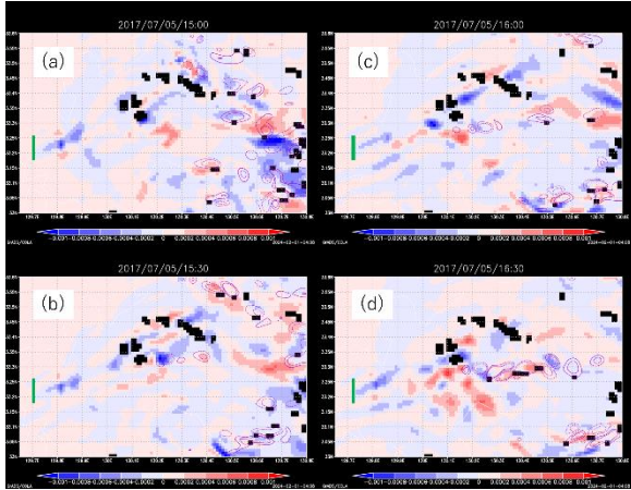
Fig. 5-5 Difference of water vapor mixing ratio [ \text{kg kg}^{-1} ].
