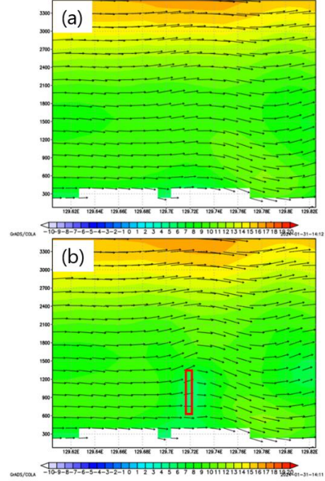
Fig. 4-3: Upper figure is without wind field manipulation; lower figure is with curtain. The vectors are the two components of wind speed in the east-west and vertical directions, and the shading is also the wind speed in the east-west. The area enclosed by the red square is the area that was manipulated in this calculation.
