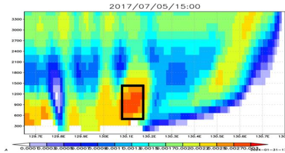
Fig. 4-6: Same as Fig. 4.5, but with the black square which indicates the domain of the initial points of the tracers.
