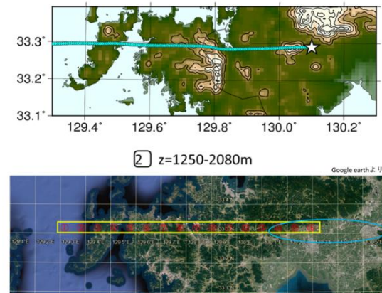
Fig. 4-8: The results of the backward flowline tracking in the lower layer together with the actual topographic data; the contour lines are filled in every 100 m, starting at 200 m. The figure below shows an image of the wind field operation locations in the lower level and their numbering.
