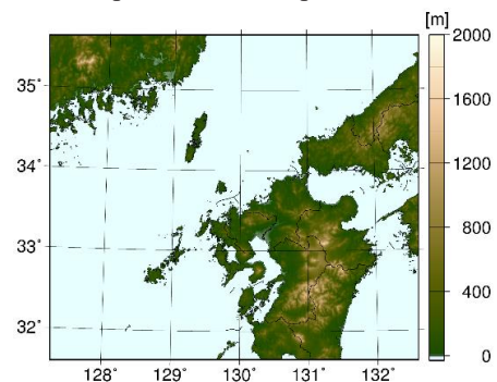
Fig. 3-1 The computation domain of CReSS
