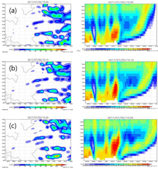
Fig. 4-5: The left figure of (a) shows rainfall intensity, the right figure are vertical section showing domain perturbation of water vapor mixing ratio ( q_v ) at 1500 JST. Water vapor tends to be basically higher at lower elevations and lower at higher elevations. (b)-(c) are same as (a) but at 1510, 1520 JST, respectively. Therefore, to quantitatively know which location has more water vapor for all altitudes, q_v , the water vapor mixing ratio minus the regional altitude average of the water vapor mixing ratio, was used as an indicator.
