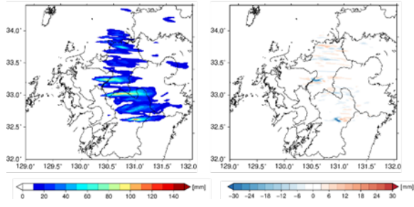
Fig. 5-1 Lefthand side figures indicate the 3-h accumulated rainfall with wind field manipulation, and righthand side figures show the difference between manipulation experiments and control run (without manipulation)
