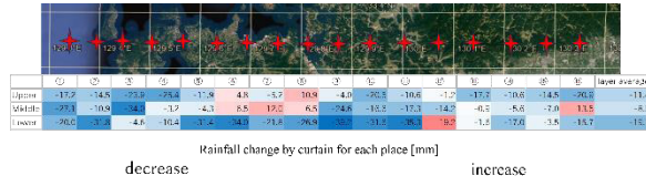
Fig. 5-2 Difference in spatial maximum peak values of 3-hour accumulated rainfall [mm] within the rainfall area in the sensitivity experiment for the wind field manipulation operation location. Positive value means increase by manipulation, negative value means decrease by manipulation.
