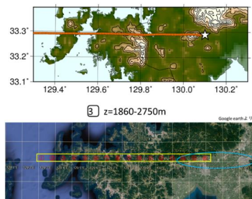
Fig. 4-10: The results of the backward trajectory line tracking in the upper layer together with the actual topographic data; the contour lines are filled in every 100 m, starting at 200 m. The lower figure shows an image of the wind field operation locations in the upper layer and their numbering.
