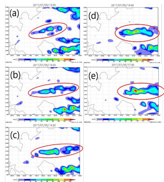
Fig. 3-2 The rainfall intensity from the initiation of the line shaped convective system at (a) 15:40, (b)16:00, (c)16:20, (d) 16:40 (e) 17:00
