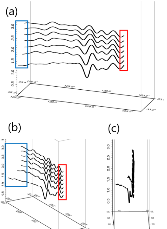
Fig. 4-7: The result of back trajectory. (a) is the result seen from south-south-east. (b) is seen from east-southeast. (c) is seen from east.
