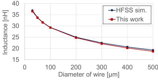
FIGURE 13. Comparison of the self inductance of the sense coil whose diameter is 10 mm and the diameter of the wire is changed from 30 \mu\text{m} to 500 \mu\text{m} .
