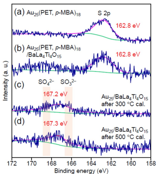
Figure 5. Comparison of S 2p XPS spectra: a) Au 25 (PET, p -MBA) 18 , b) Au 25 (PET, p -MBA) 18 /BaLa 4 Ti 4 O 15 , Au 25 /BaLa 4 Ti 4 O 15 obtained by calcination at c) 300 °C and d) 500 °C. In the spectra, the green and purple lines indicate the baseline and fitting result, respectively. The peak at ca. 162.8 eV is assigned to S in Au–S, whereas the peaks at ca. 167.2 eV and ca. 167.3 eV are assigned to S oxides, such as SO 3 2- and SO 4 2- .
