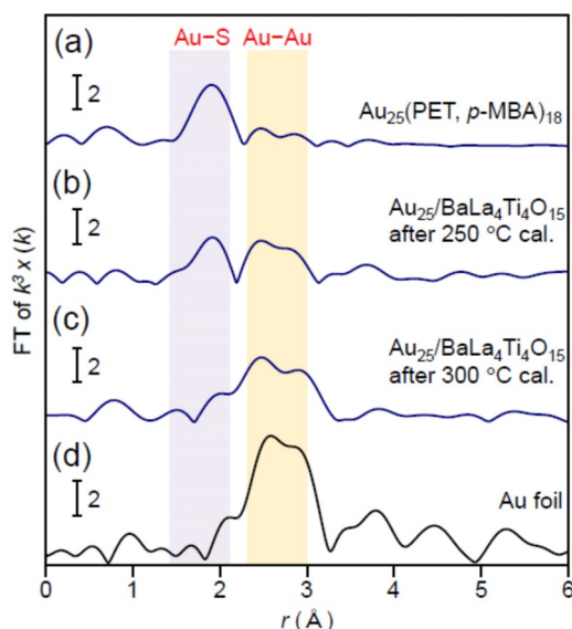
Figure 4. Au L 3 -edge FT-EXAFS spectra of a) Au 25 (PET, p -MBA) 18 , Au 25 /BaLa 4 Ti 4 O 15 obtained by calcination at b) 250 °C and c) 300 °C, and d) Au foil. The purple and yellow regions indicate the Au–S and Au–Au bond regions, respectively. [43,47] In (a), only weak peaks appear in the Au–Au bond region because the Au 13 core (Scheme S2(a)) fluctuates at room temperature. [48]
