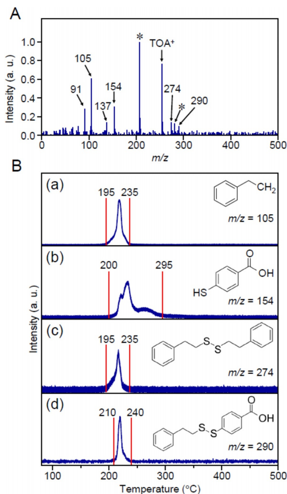
Figure 1. A) DIP-MS spectrum of compounds desorbed from \text{Au}_{25}(\text{PET}, p\text{-MBA})_{18} in the temperature range of 80\text{--}500^\circ\text{C} . In this spectrum, the peaks with an asterisk (*) are not due to the sample but to compounds deposited in the apparatus. B) Temperature dependence of each mass peak: a) PE ( m/z = 105 ), b) p\text{-MBA} ( m/z = 154 ; not thiolate but thiol), c) (\text{PET})_2 ( m/z = 274 ), and d) PET- p\text{-MBA} ( m/z = 290 ).
