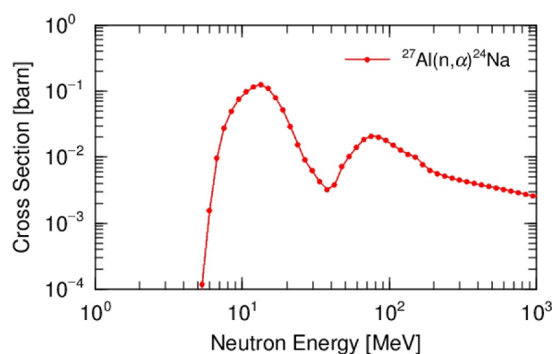
Figure 6. Cross-sections of activation reaction for aluminum.
