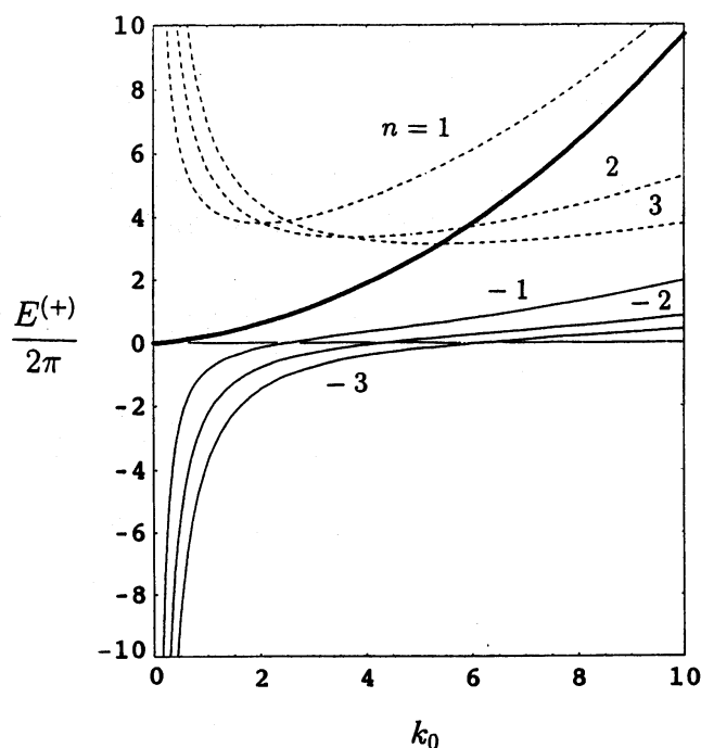
Figure 1: The wave energy E^{(+)} , normalized by 2\pi , of the the bending wave with m = 1 as functions of k_0 , as given by (5.7). The solid thick line corresponds to the primary mode, solid lines to the retrograde higher radial modes, and dashed lines to the cograde higher radial modes.
