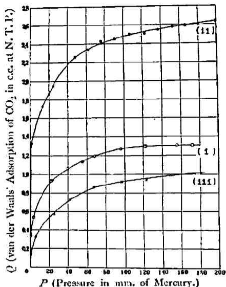
Fig. 4. Isotherms for the Adsorption of Carbon Dioxide by Reduced Iron at 0°C. The Relation between the Chemisorption and van der Waals' Adsorption.
