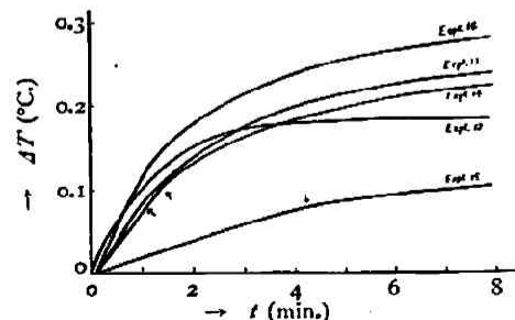
Fig. 13.—[NaHSO 3 ] and [KIO 3 ] are not equivalent.
