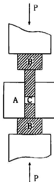
Fig. 1 Diagram of the pressure apparatus A : pressure vessel B : pistons C : sample region
