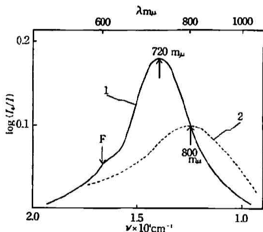
Fig. 1 Quenching effect on the absorption spectrum of color centers in NaI specimen produced by electrolysis at 600°C
