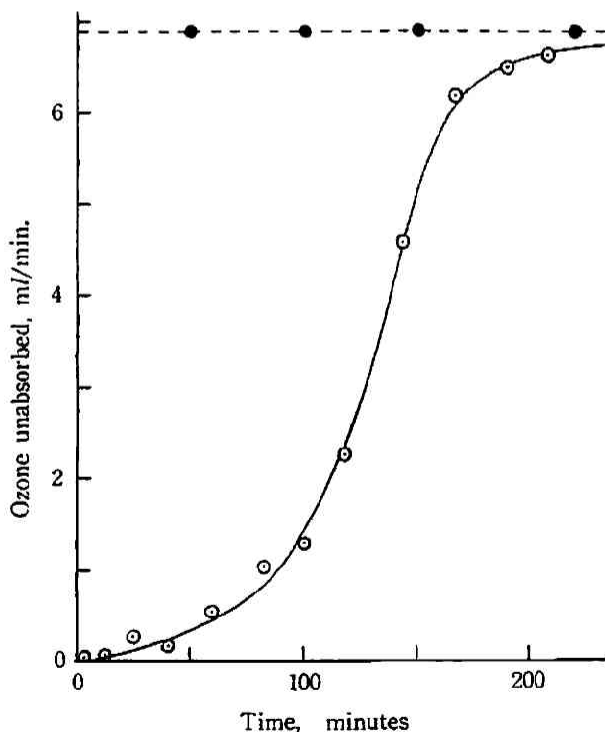
Fig. 3 Ozonation of oleic acid and its urea adduct by flow method at 15^\circ\text{C}
