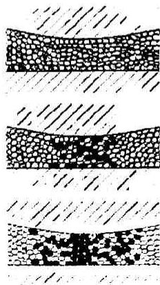
Fig. 10. Binary mixture of dielectric powders at the loading F_1 < F_2 < F_3 :
