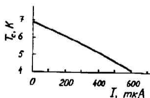
Fig. 17. Critical temperature of superconducting transition in xenon versus current intensity.
