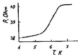
Fig. 15. The superconducting transition in gallium phosphide.
