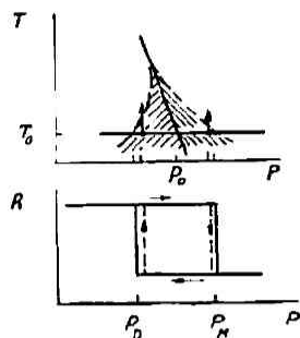
Fig. 2. The scheme of "unfreezing" of metastable phases : a) the part of phase P - T diagram ; b) the resistance vs. load curve. The dashed lines correspond to the "unfreezing" processes under heating of the sample.
