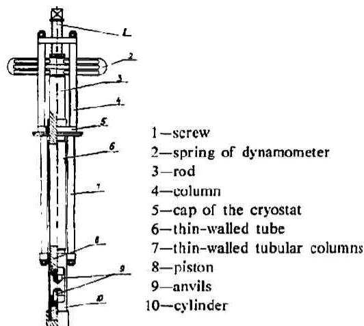
Fig. 5. The scheme of low-temperature press.
