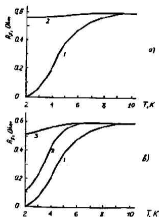
Fig. 19. The superconducting transition in NaCl sample at various values of current intensity: a) 1 - I = 100 mA; 2 - I = 500 mA; and various values of magnetic field intensity b) I = 100 mA; 1 - H = 0 ; 2 - H = 12 kOe; 3 - H = 24 kOe.
