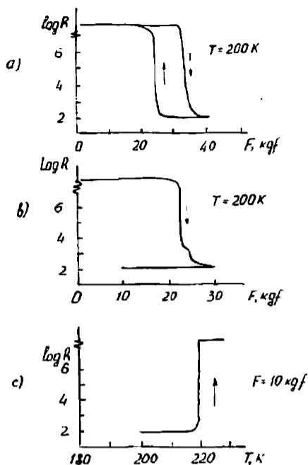
Fig. 7. The dielectric-to-metal transition in H 2 O sample and the "unfreezing" of metastable metallic phase.
