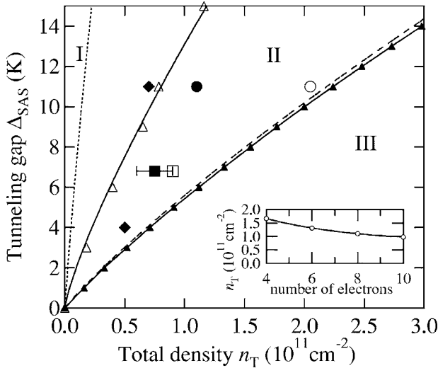
FIG. 7. Phase diagram in the n_T - \Delta_{\text{SAS}} plane at the balanced point. The solid and open circles are the S(I)-CAF(II) and CAF(II)-F(III) phase transition points derived from the data in Fig. 2, respectively. The open square is a reinterpreted S-CAF phase boundary, while the error bar on the solid square shows that the CAF-F phase boundary must be within this region, as estimated from Ref. 19. The solid diamonds are reinterpreted S-CAF phase boundary determined from the SCAF-FCAF region boundary appeared in Ref. 21. See details in the text. The dotted line and dashed line are the calculated S-CAF and CAF-F phase boundaries by the Hartree-Fock approximation. Open triangles and solid triangles are the calculated S-CAF and CAF-F phase boundary points by an exact diagonalization method. Inset: Convergence of the ED method. The total density n_T at the CAF-F transition point vs the number of electrons to be diagonalized for \Delta_{\text{SAS}}=11 K.
