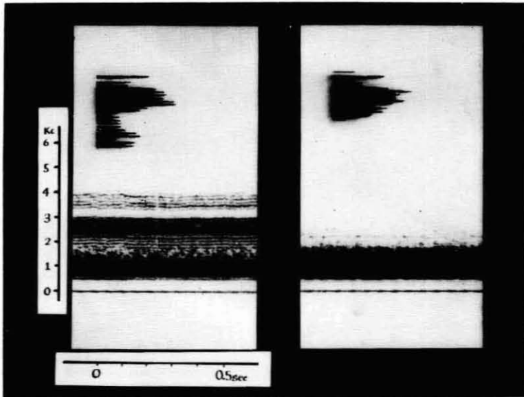
Fig. 5. Soundspectrogram of vowels "e" plus band noise test sound showing the status of synthesis. Bandwidth of filter and mean of rating indicated under corresponding sound.
