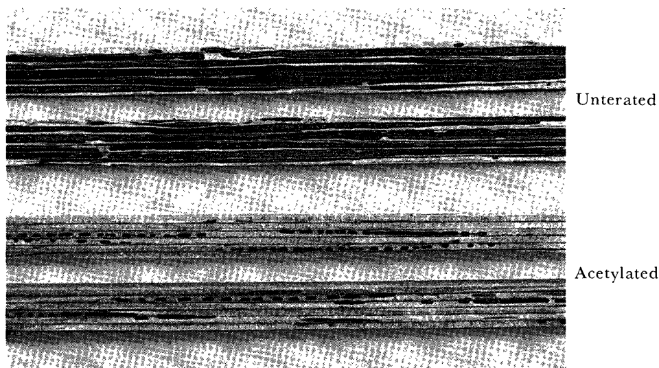
Fig. 1. Untreated and acetylated Douglas-fir LVLs exposed to attack by termites of C. formosanus for 30 days on the breeding nest. Size of specimen is 20×20×300 mm.
