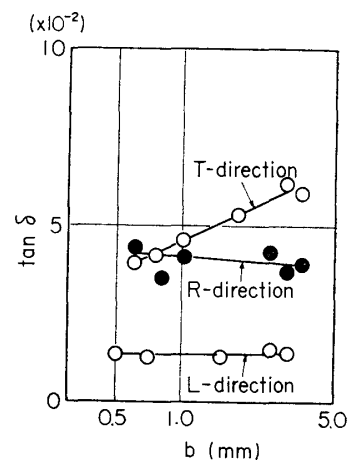
Fig. 24. The dependence of the annual ring width b on \tan \delta of Sitka spruce at 60 kHz.
