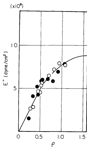
Fig. 17. The relation between E'' and \rho in radial direction at 60 kHz. The open circles and solid line represent the untreated wood, and the closed circles represent the extracted wood.
