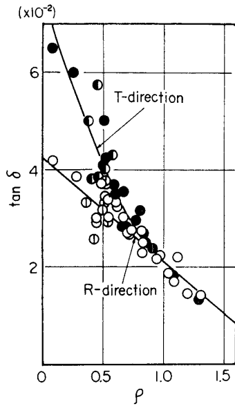
Fig. 9. The relation between \tan \delta and \rho in the transverse direction at 60 kHz. \circ hardwood in R-direction, \ominus softwood in R-direction, \bullet hardwood in T-direction, \bullet softwood in T-direction.
