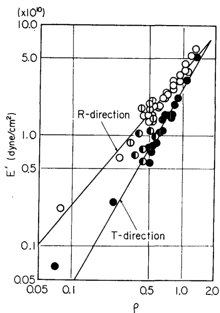
Fig. 4. The relation between E' and \rho in the transverse direction at 60 kHz. \circ hardwood in R-direction, \odot softwood in R-direction, \bullet hardwood in T-direction, \bullet softwood in T-direction.
