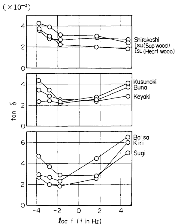
Fig. 3 (b). tan δ as a function of frequency in tangential direction.
