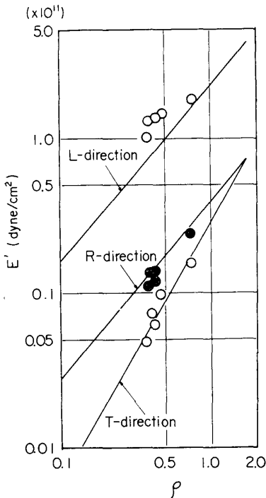
Fig. 19. The relation between E' and \rho at 60 kHz. The circles represent the wood used for the musical instruments, and solid lines represent regression lines of Figs. 4 and 12.
