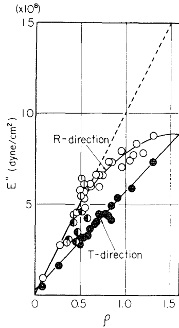
Fig. 6. The relation between E'' and \rho in the transverse direction at 60 kHz. \circ hardwood in R-direction, \odot softwood in R-direction, \bullet hardwood in T-direction, \ominus softwood in T-direction.
