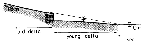
Fig. 7 A N-S profile showing a theoretical flood level on the Old and Young deltas. Notice that the flood depth is deepest just in front of the scarp separating the Old delta and Young delta
