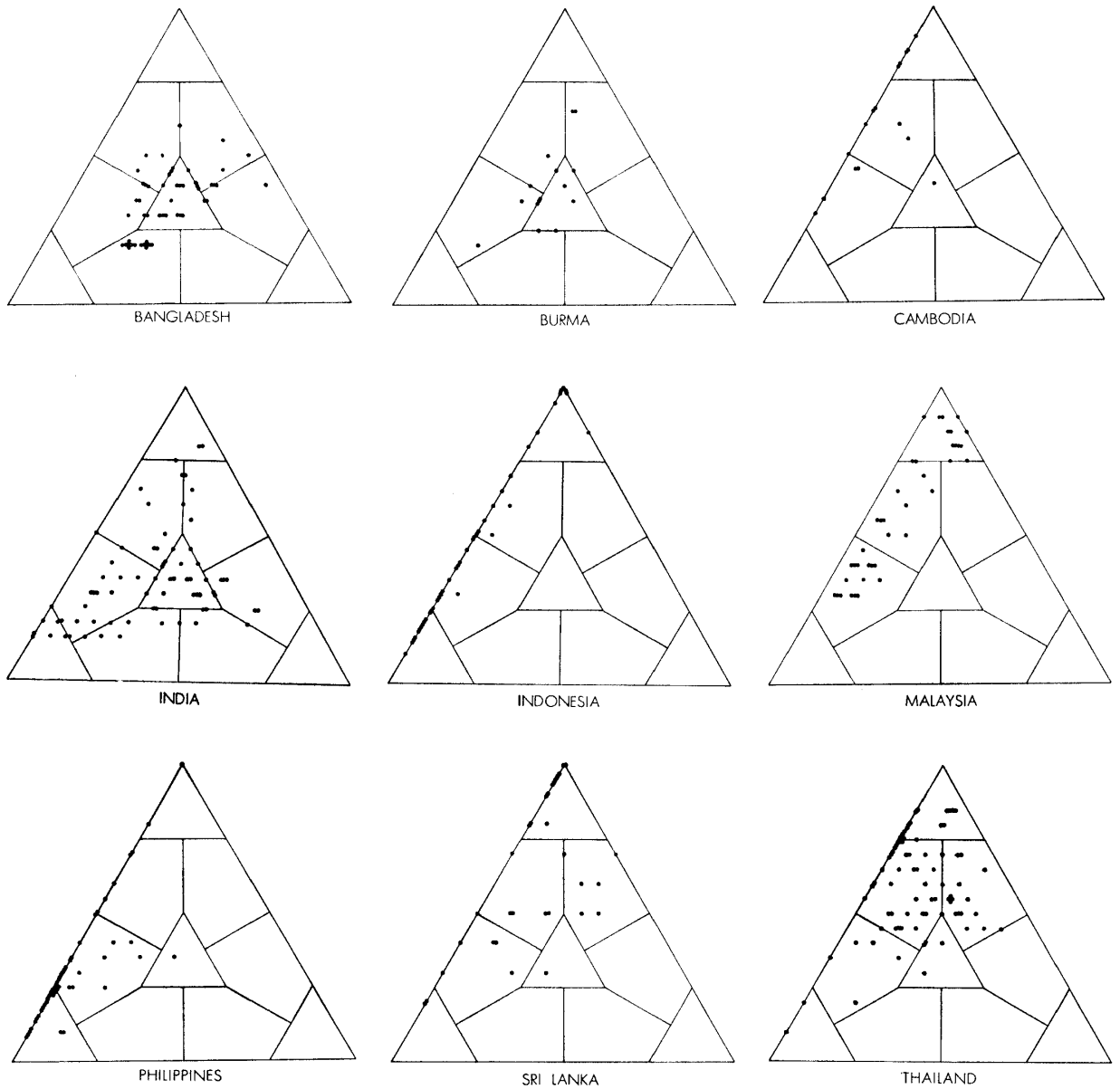
Fig. 4 Distribution of sample soils in the triangular diagram for grouping clay mineral compositions by countries.
