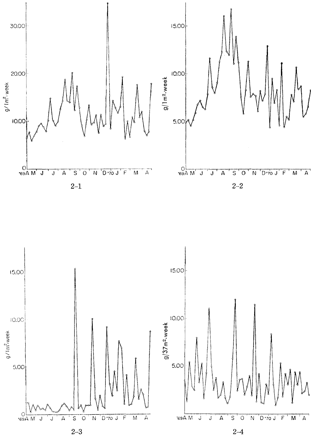
Fig. 2-1~4 Weekly amount of various kind of litter fall for one year at 1 ha-plot. Further notice, see text.
