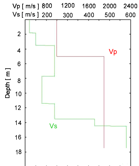
Fig. 4.5: Graph of the PS logging data. This graph is plotted by Tab. 4.1
