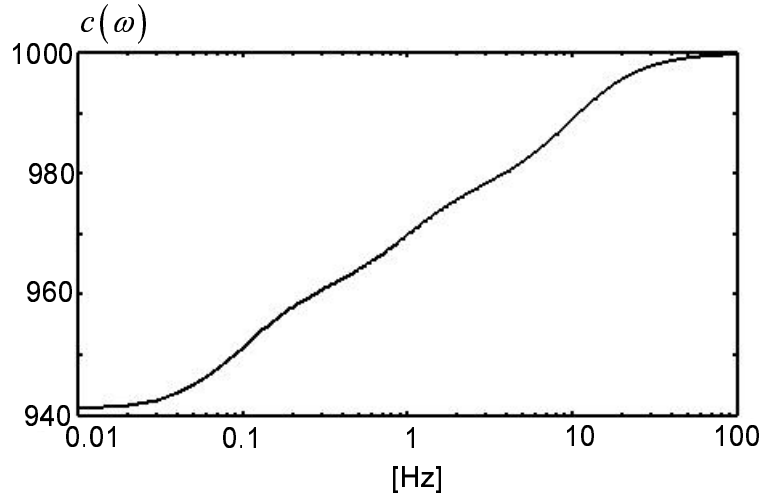
Fig. 2.5: Phase velocity by SLSM with 3 relaxation mechanisms. This graph is obtained from Table 2.1, Eq. (2.71) and c(\infty) = 1000 .
