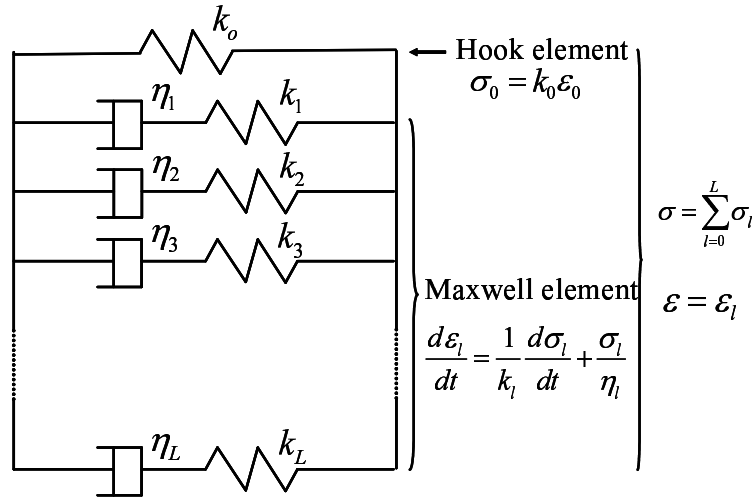
Fig. 2.3: SLSM; Standard Linear Solids Model. This is a rheologic model for explaining constant Q behavior.
