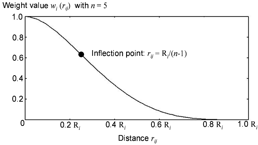
Fig. 3.5: A weight function for moving least square. This graph is obtained by Eq. (3.70) with n = 5
