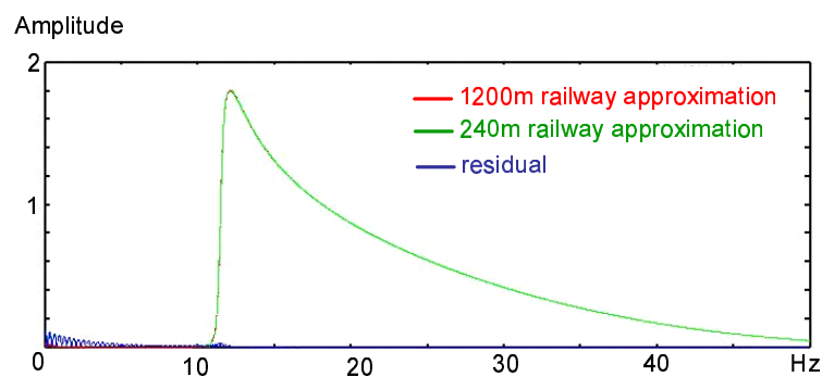
(c) 240 m railway approximation
