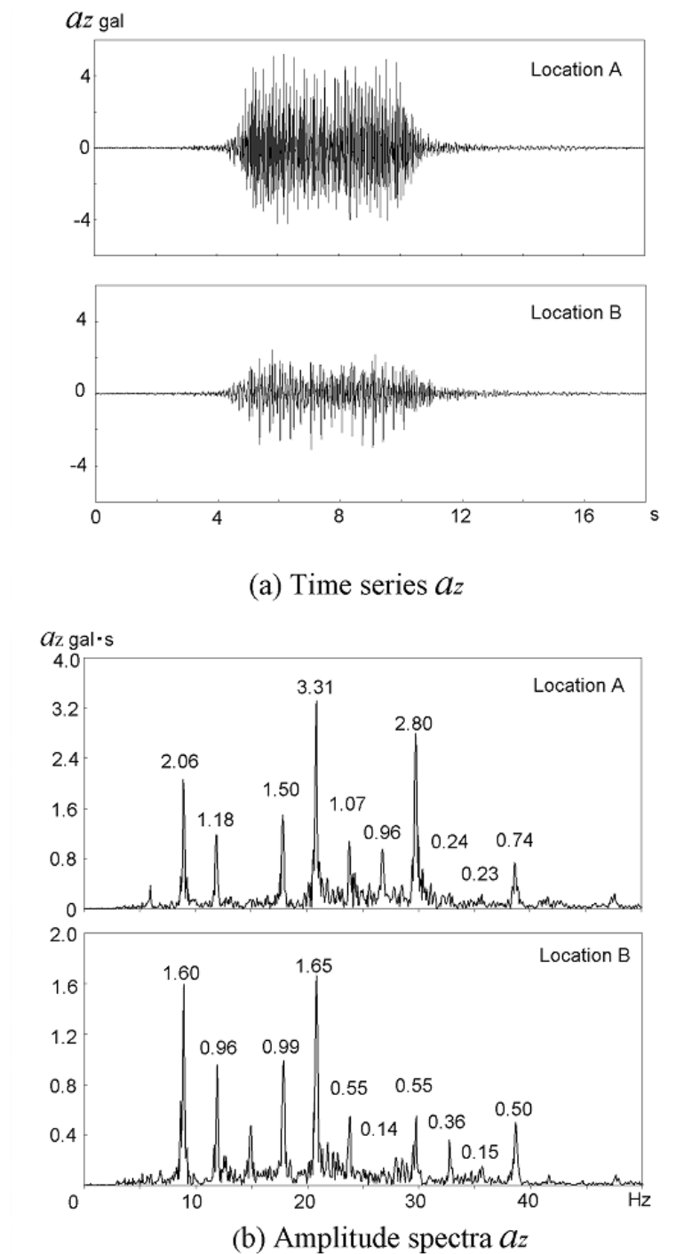
Fig. 4.6: Ground vibration observed at a field site. (a) Time series for field records of vertical components of acceleration. Locations A and B are 15 m and 30 m from the rail track, respectively. (b) Amplitude spectra for (a). Ten peak frequencies are indicated and are at 8.9, 11.9, 17.9, 20.8, 23.8, 26.8, 29.7, 32.7, 35.6, and 38.6 Hz.
