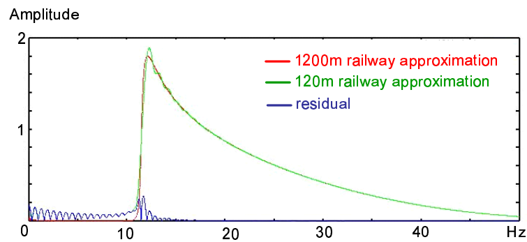
(b) 120 m railway approximation
