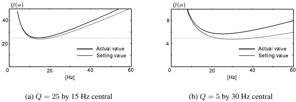
Fig. 2.6: A comparison between setting and actual value in Blanch method.
