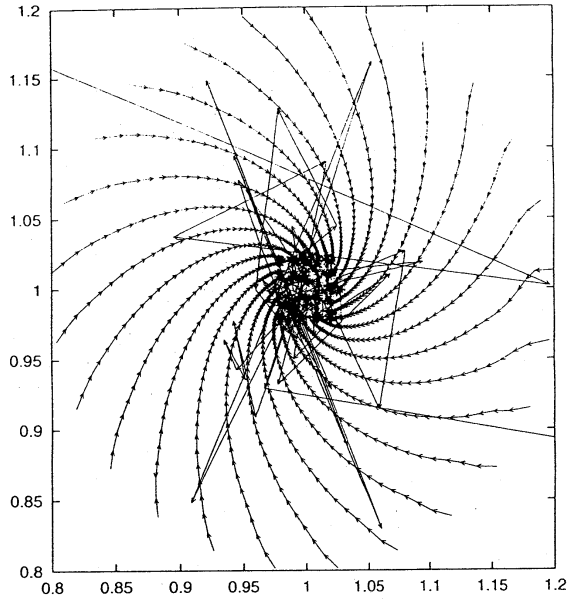
图 13. SOR (1.6), \omega = 1.8 .
