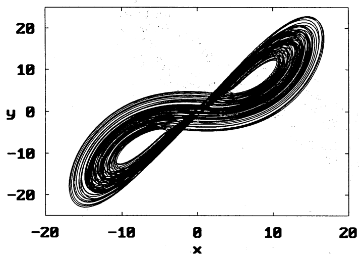
Figure 1. Projection of the attractor \mathcal{A}_Q , Q = 0.5 .
