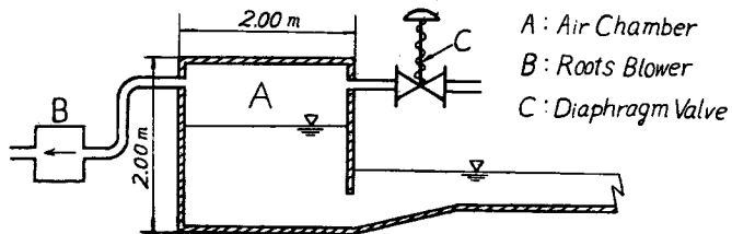
Fig. 1. Experimental facilities.
