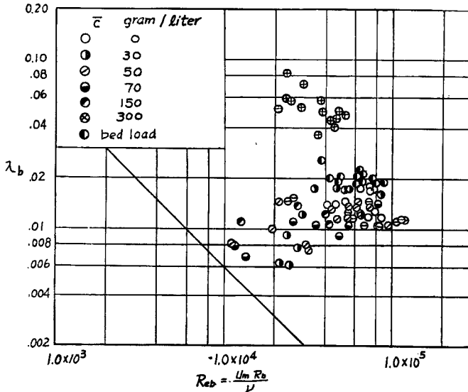
Fig. 7. Correlation between \lambda_b and R_e
