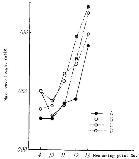
Fig. 8 Variations of maximum wave height ratio
