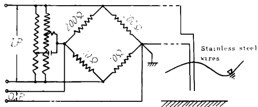
Fig. 3 Circuit diagram of sensing element of wave recorder
